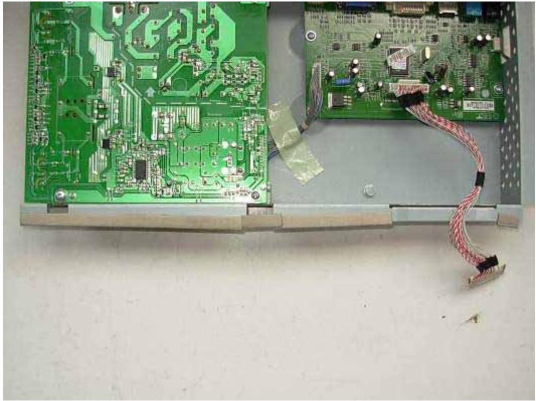
FIGURE 19 LCD MONITOR (M/N: W2442PAT) DEBUG 2
