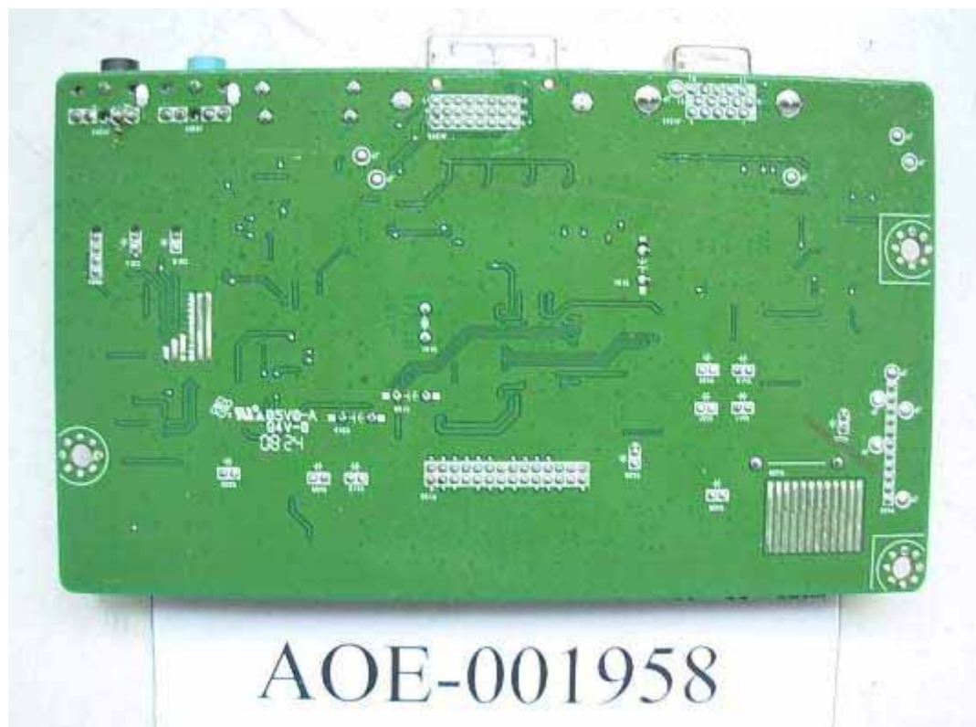
FIGURE 8 LCD MONITOR (M/N: W2442PAT) MAIN BOARD (SOLDERED SIDE)
