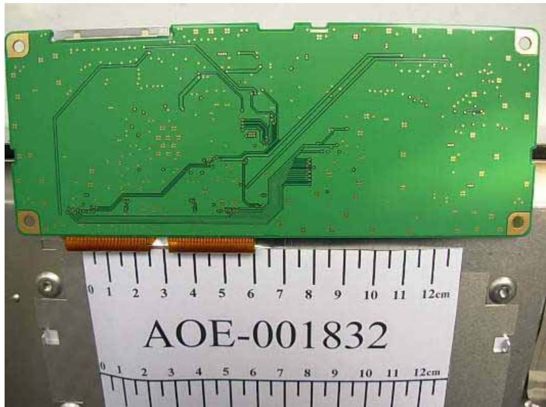
FIGURE 18 LCD MONITOR (M/N: W2452SQT) LCD PANEL MAIN BOARD (SOLDERED SIDE)
