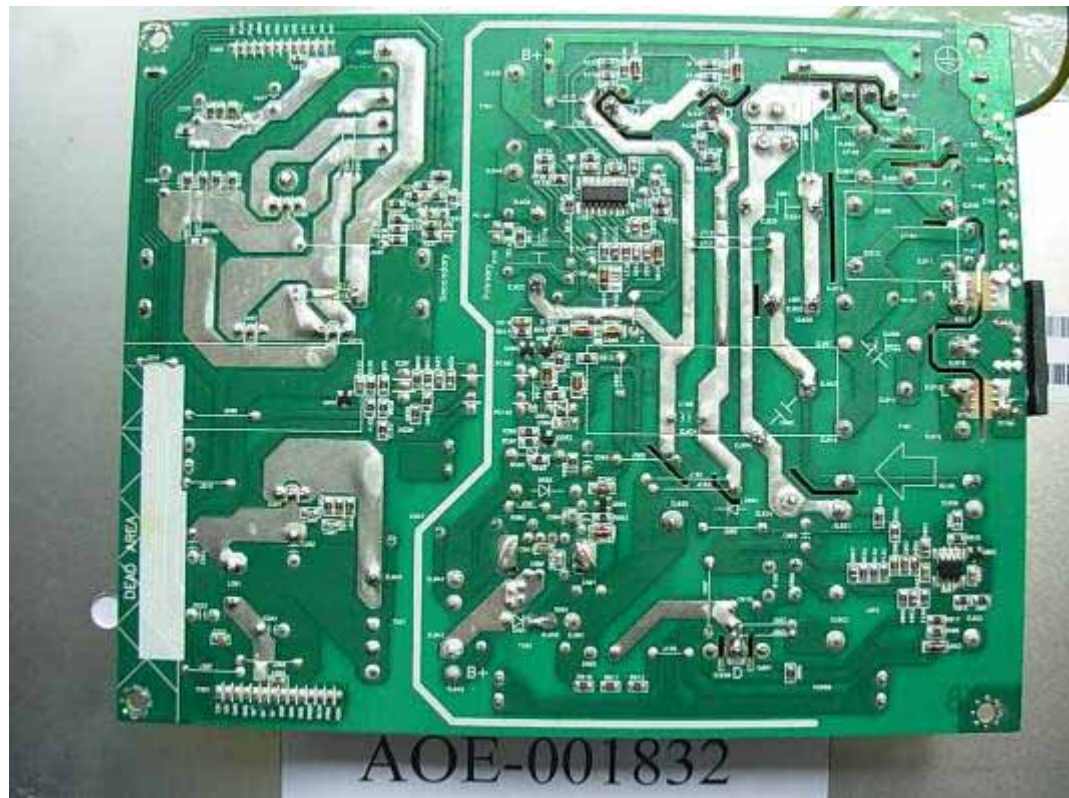
FIGURE 8 LCD MONITOR (M/N: W2452SQT) POWER BOARD (SOLDERED SIDE)
