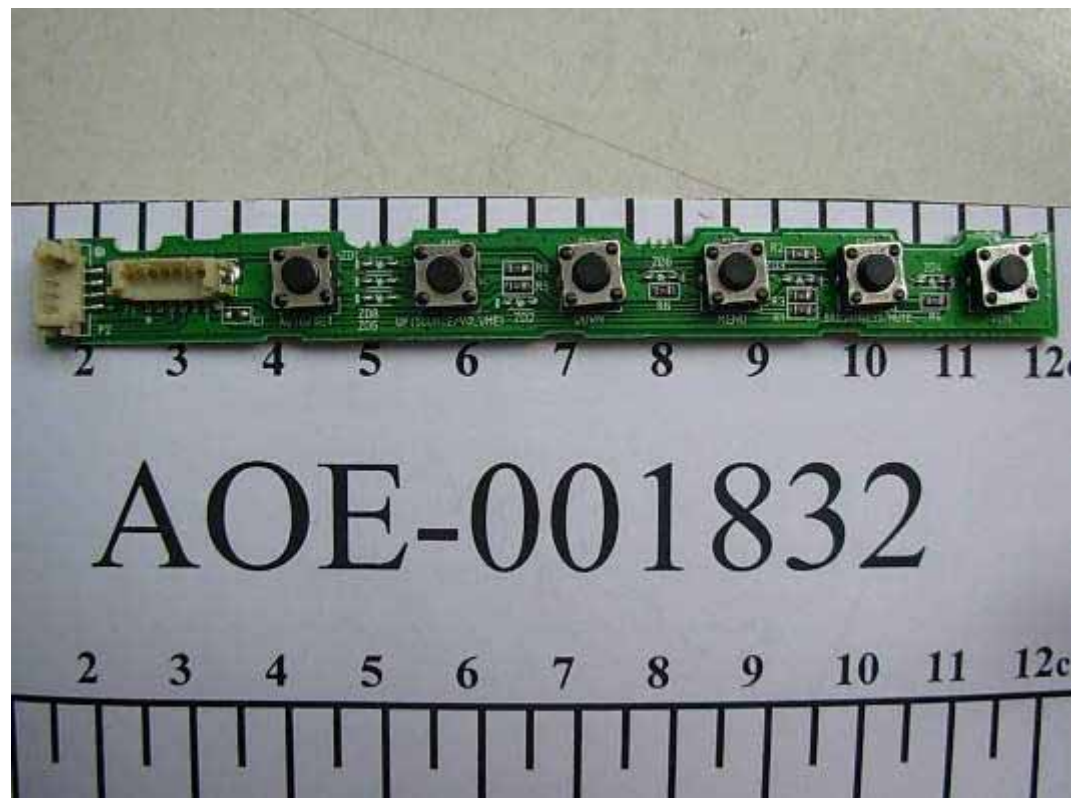
FIGURE 4 LCD MONITOR (M/N: W2452SQT) BUTTON BOARD (COMPONENT SIDE)
