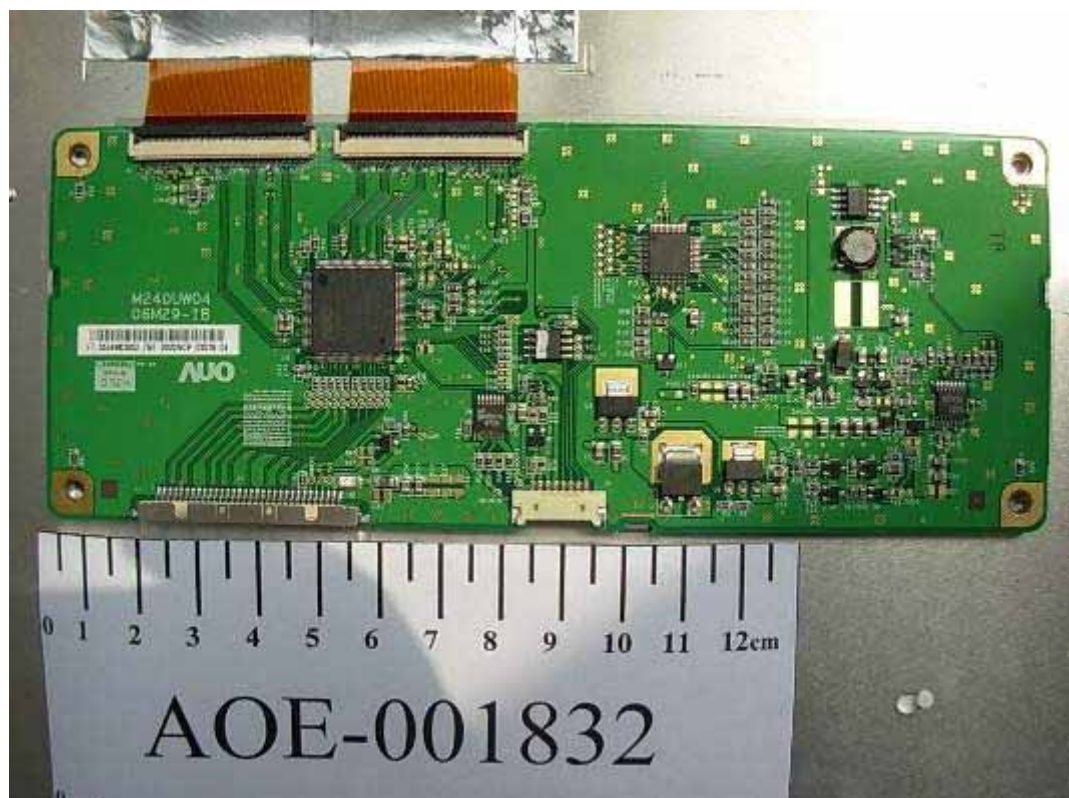
FIGURE 17 LCD MONITOR (M/N: W2452SQT) LCD PANEL MAIN BOARD (COMPONENT SIDE)
