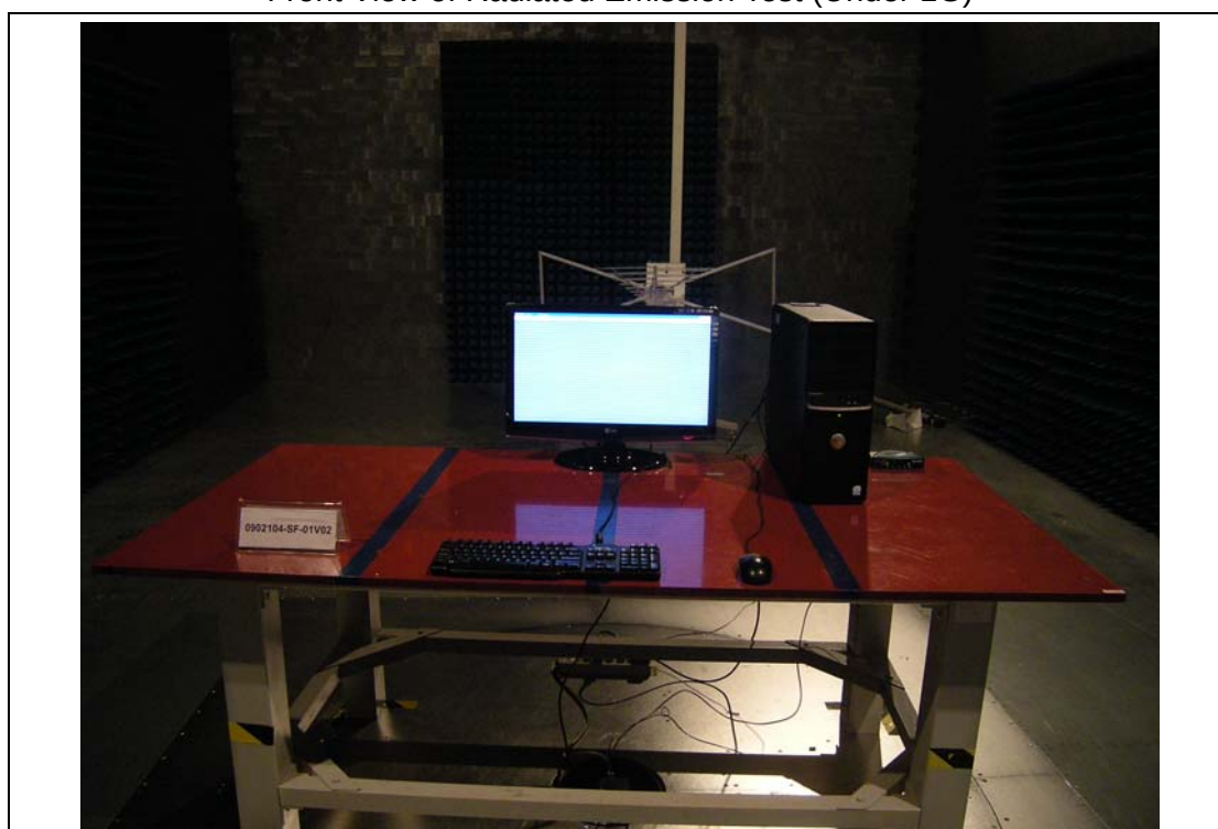
Front View of Radiated Emission Test (Under 1G)
