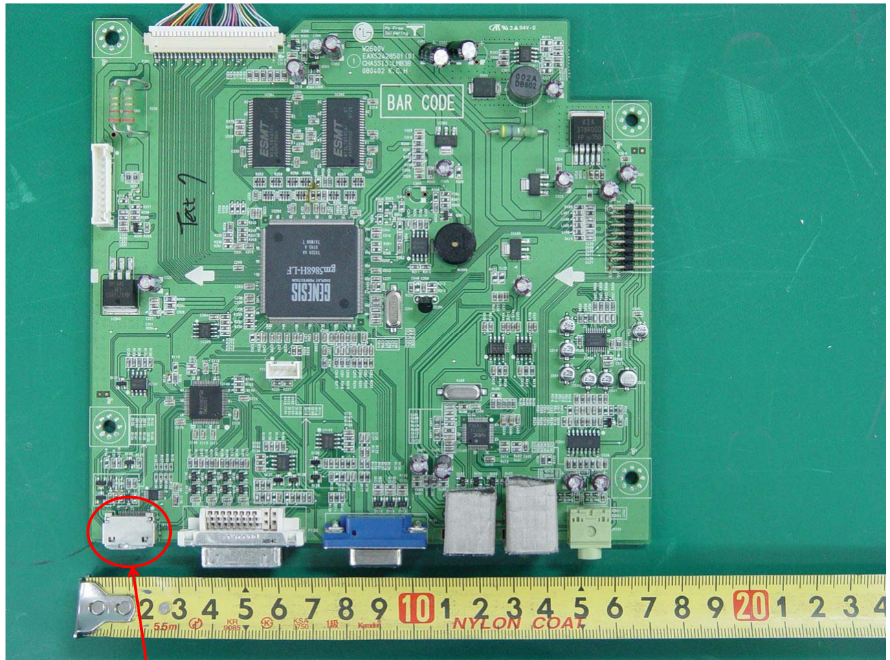
HDMI port
