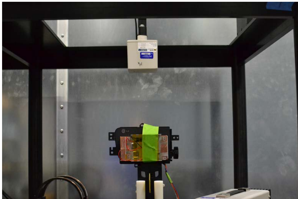
E/H Field Measurement on EUT Side "B"
