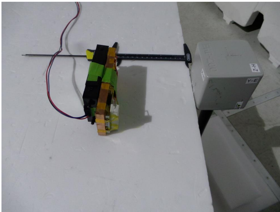
E/H Field Measurement on EUT Side "E" (15cm)
