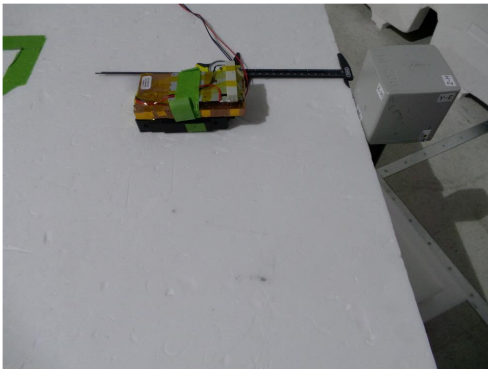
E/H Field Measurement on EUT Side "C"
