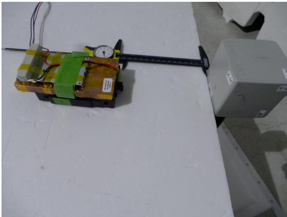
E/H Field Measurement on EUT Side "A"
