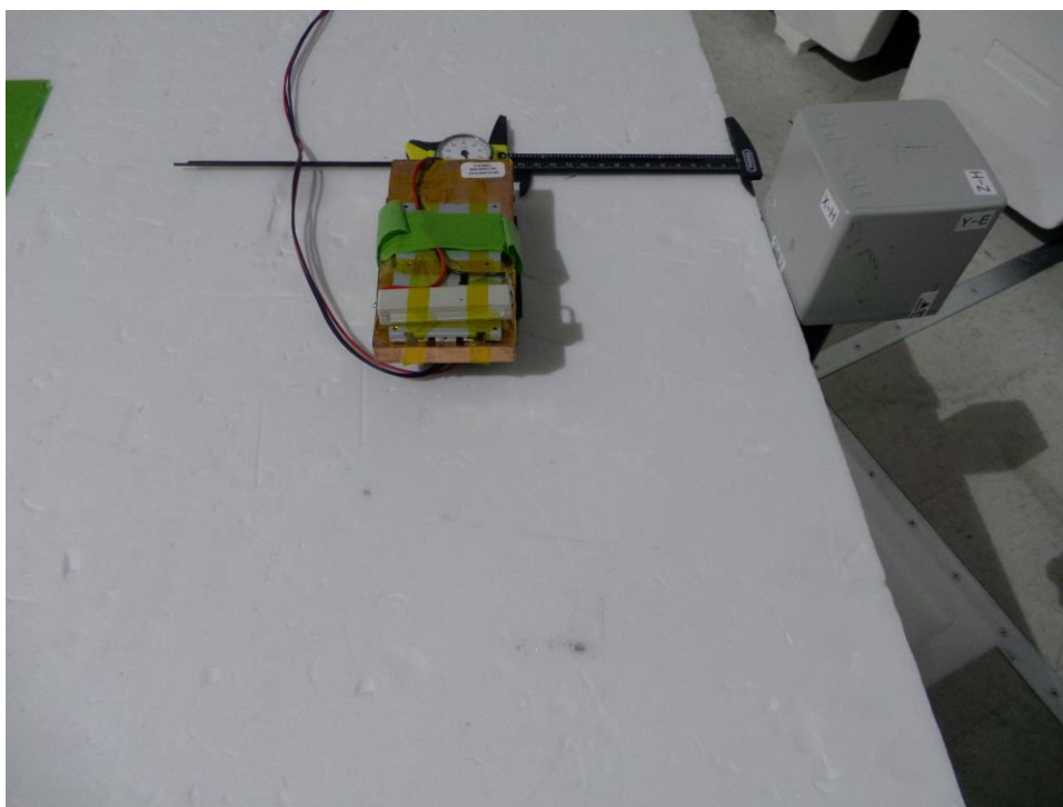
E/H Field Measurement on EUT Side "D"
