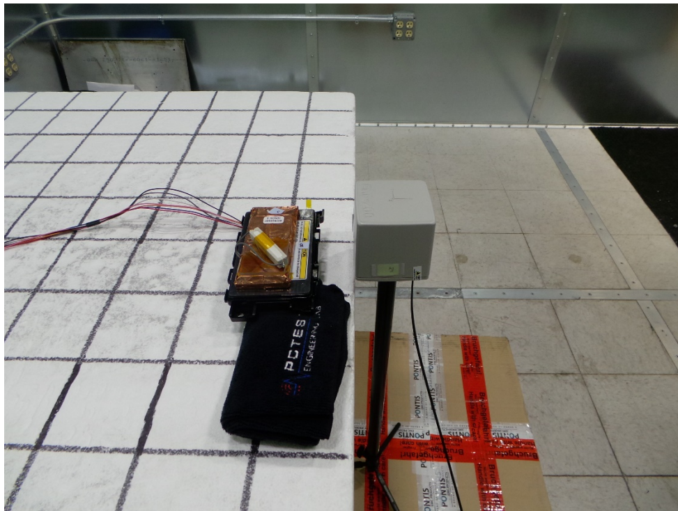
Figure 2. E-/H-Field Measurement (Position B)
