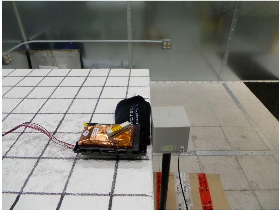
Figure 1. E-/H-Field Measurement (Position A)
