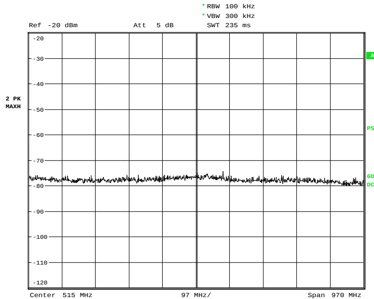
Plot 7-15. Radiated Spurious Plot above 30 MHz (Pol. H)
