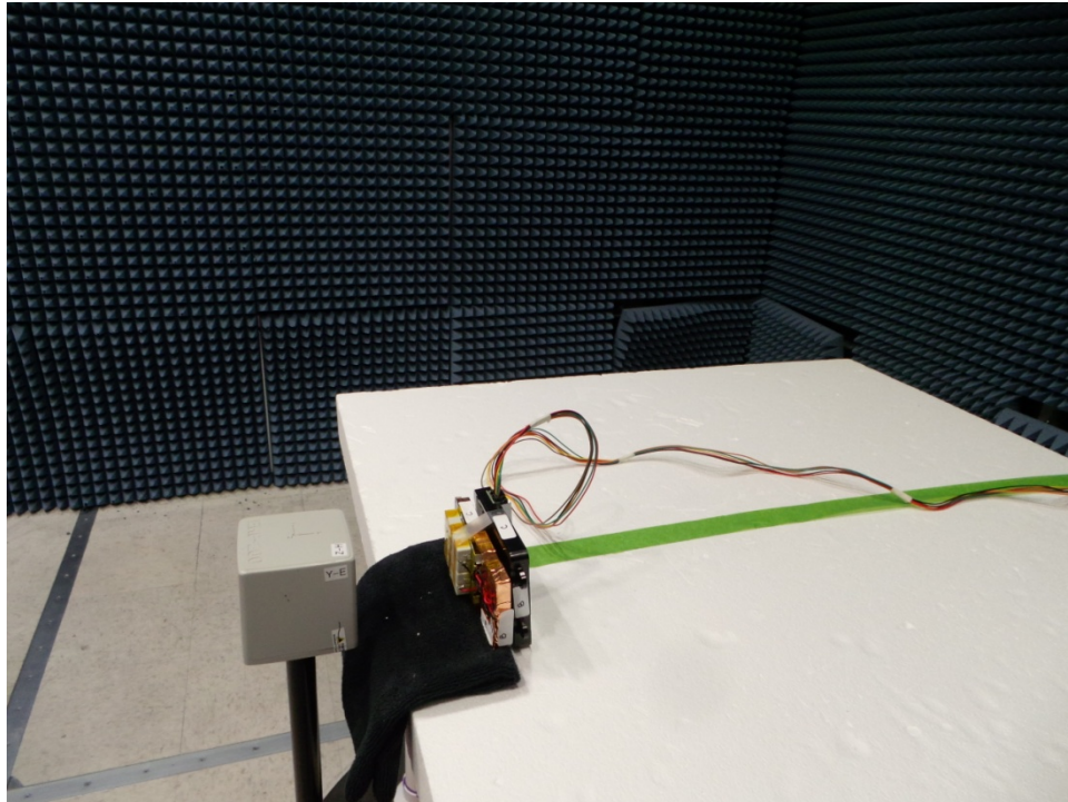
Figure 5. E-Field Measurement (Position E)
