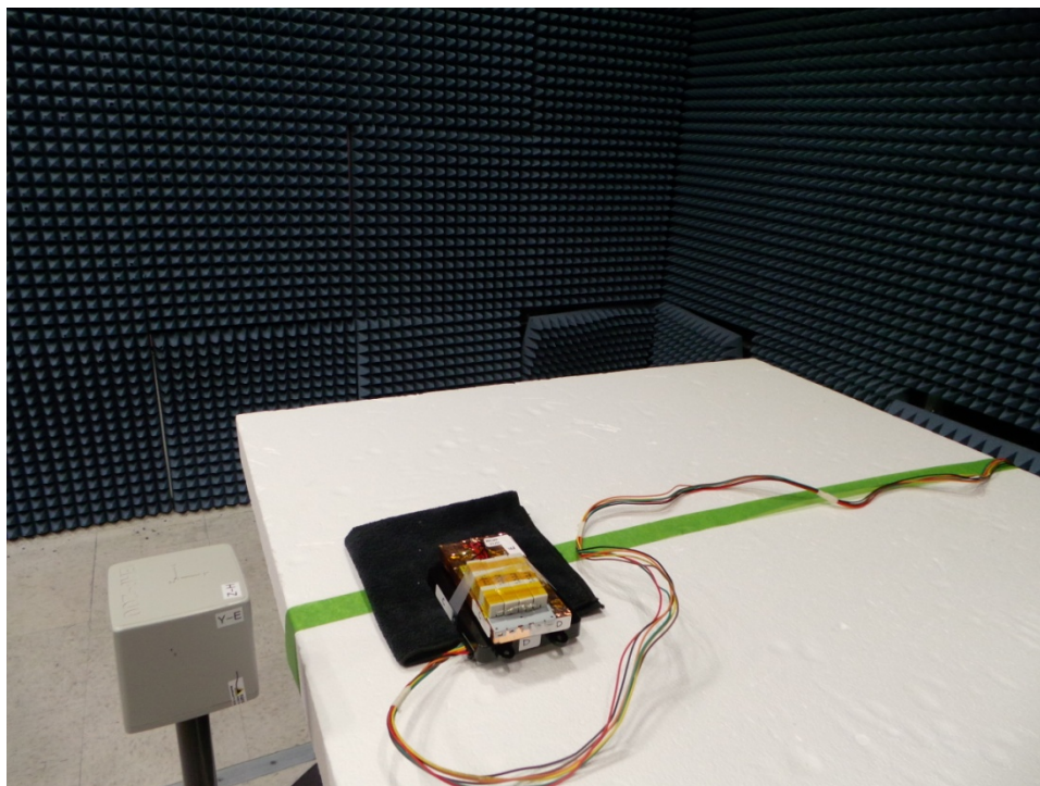
Figure 3. E-Field Measurement (Position C)
