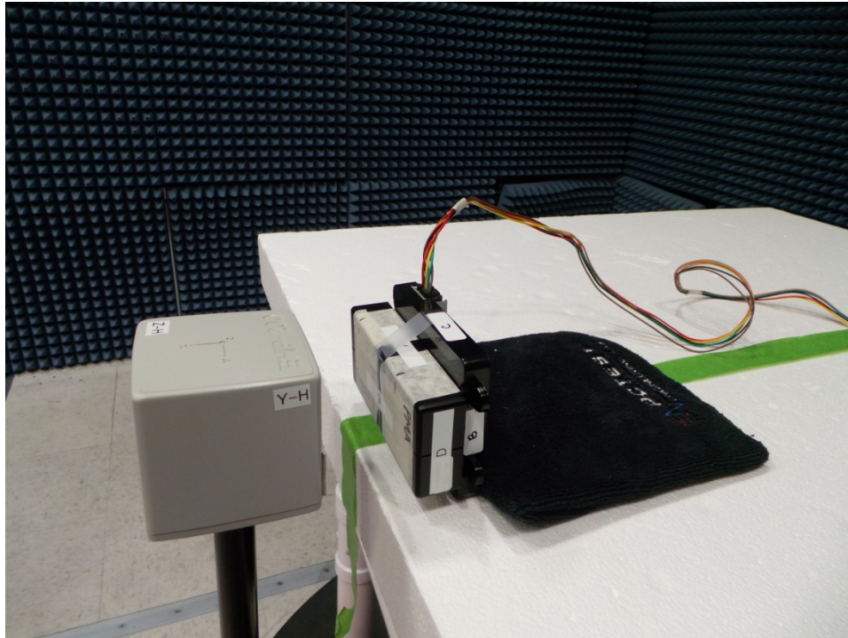
Figure 15. E-Field Measurement (Position E)
