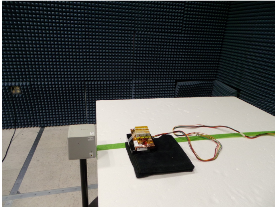
Figure 1. E-Field Measurement (Position A)
