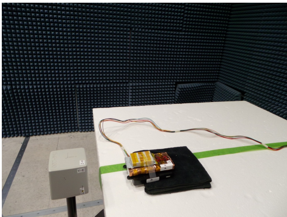
Figure 4. E-Field Measurement (Position D)
