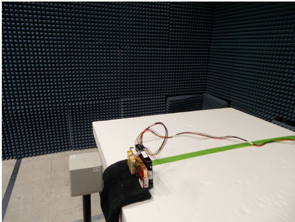
Figure 10. H-Field Measurement (Position E)
