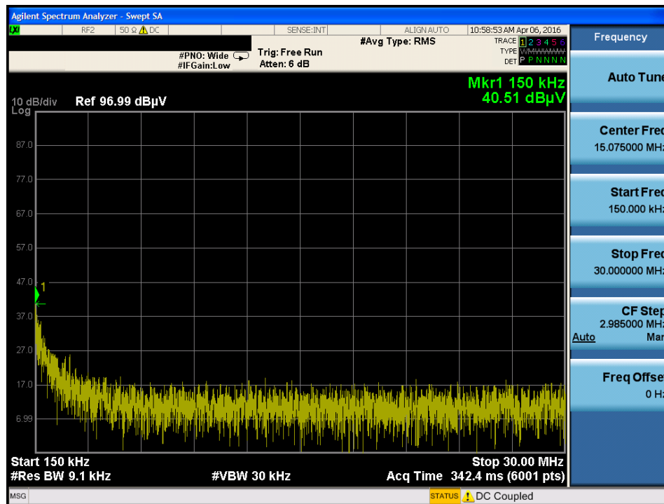
Plot 7-12. Radiated Spurious Plot below 30MHz (Pol. Y)
