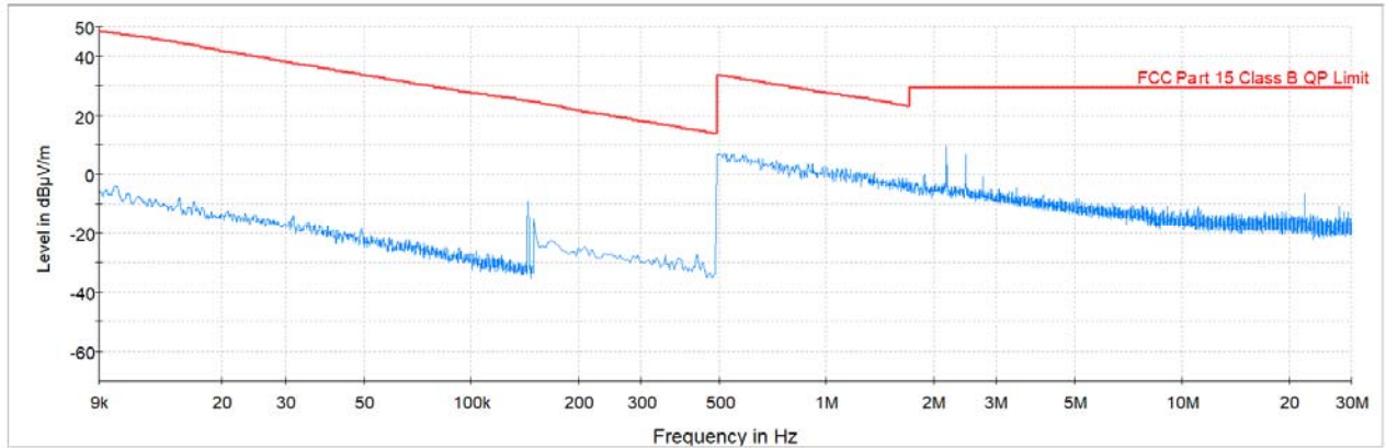
Plot 7-1. Radiated Spurious Plot from 9kHz – 30MHz (Pol. X)
