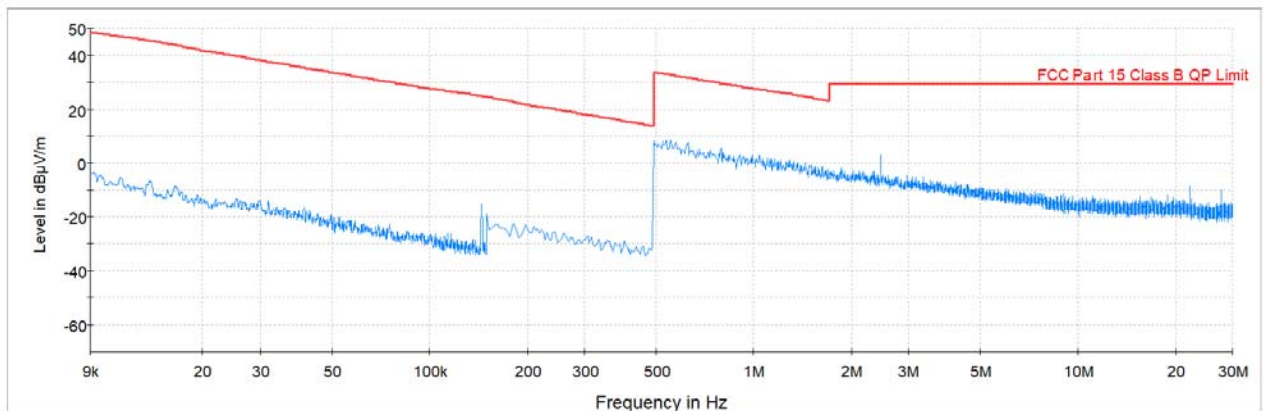
Plot 7-2. Radiated Spurious Plot from 9kHz – 30MHz (Pol. Y)
