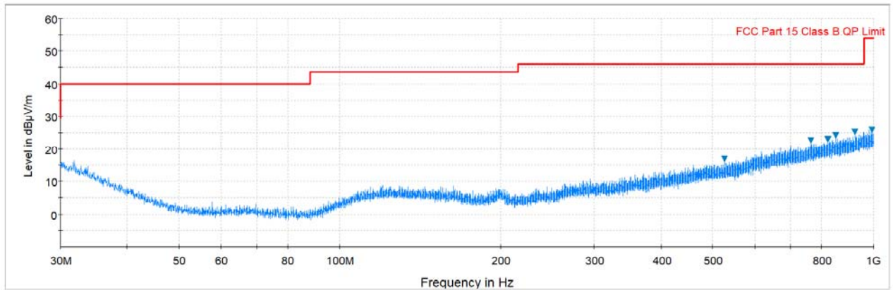
Plot 7-4. Radiated Spurious Plot above 30 MHz (Pol. H)
