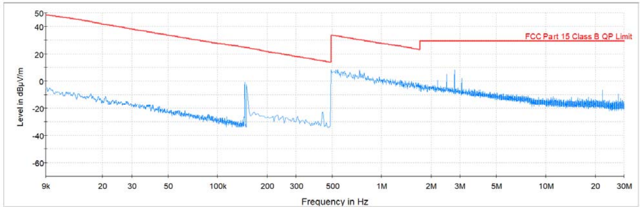
Plot 7-6. Radiated Spurious Plot from 9kHz – 30MHz (Pol. X)
