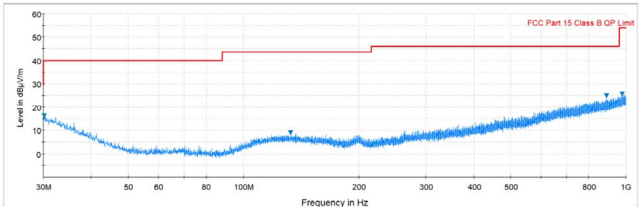
Plot 7-10. Radiated Spurious Plot above 30MHz (Pol. V)
