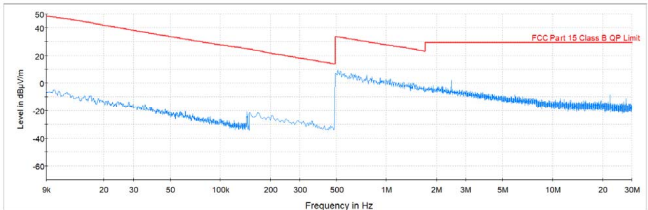
Plot 7-18. Radiated Spurious Plot from 9kHz - 30MHz (Pol. Y)
