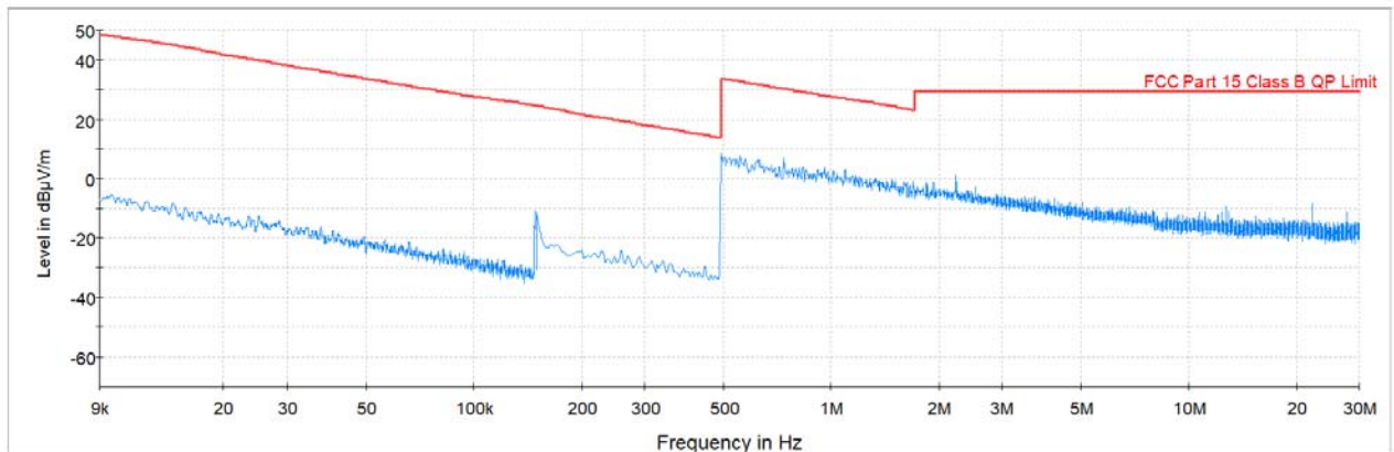
Plot 7-7. Radiated Spurious Plot from 9kHz - 30MHz (Pol. Y)
