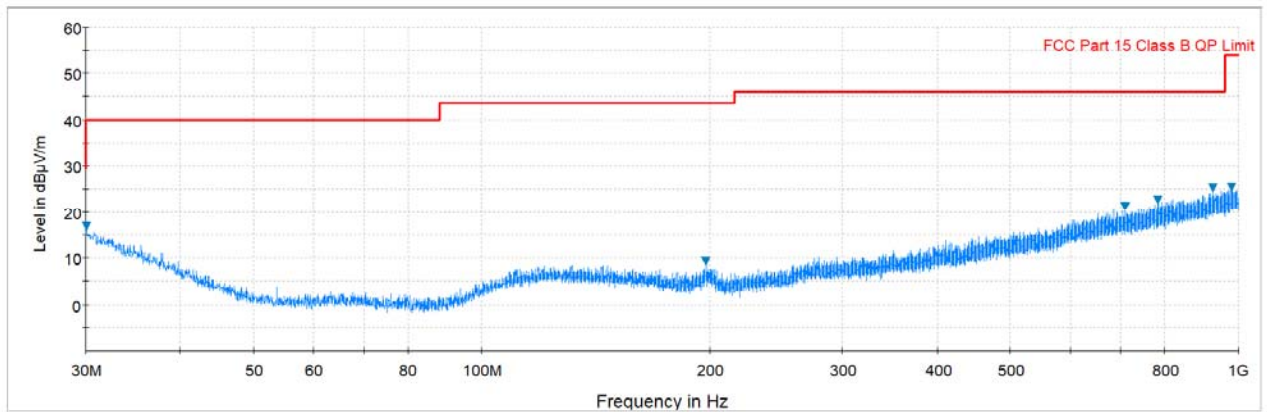
Plot 7-12. Radiated Spurious Plot above 30MHz (Pol. V)
