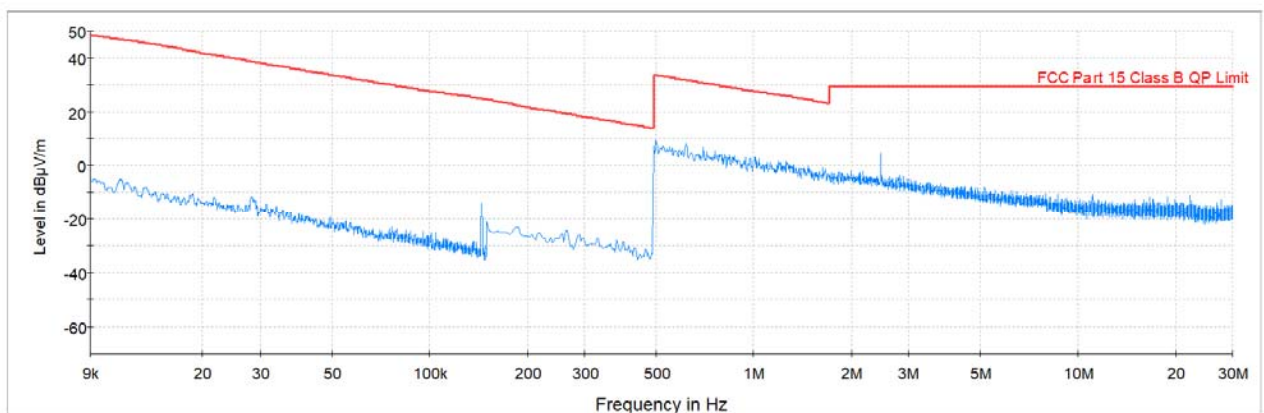
Plot 7-3. Radiated Spurious Plot from 9kHz – 30MHz (Pol. Z)
