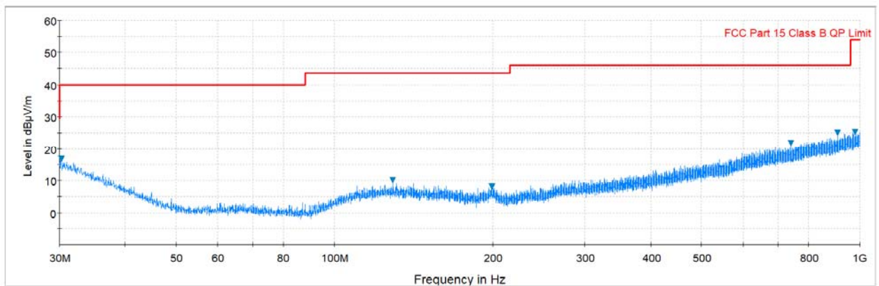
Plot 7-5. Radiated Spurious Plot above 30MHz (Pol. V)
