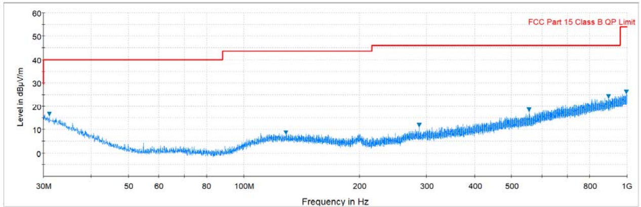
Plot 7-9. Radiated Spurious Plot above 30 MHz (Pol. H)
