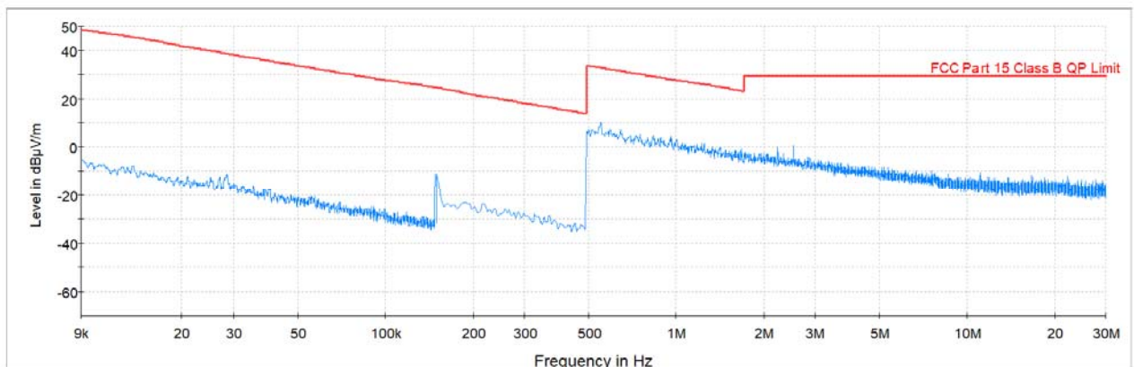
Plot 7-8. Radiated Spurious Plot from 9kHz - 30MHz (Pol. Z)
