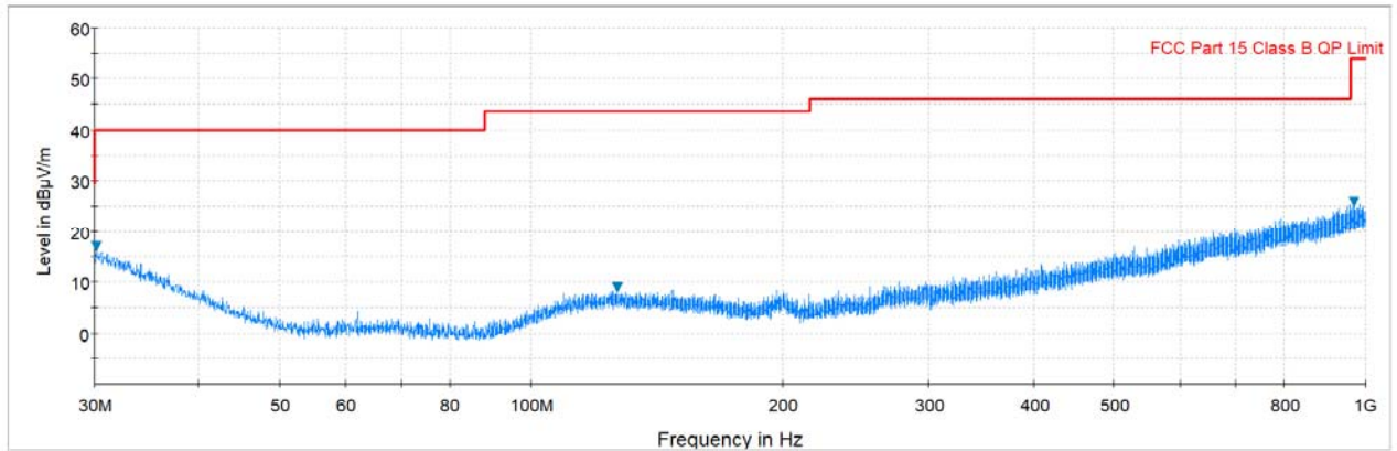
Plot 7-11. Radiated Spurious Plot above 30 MHz (Pol. H)
