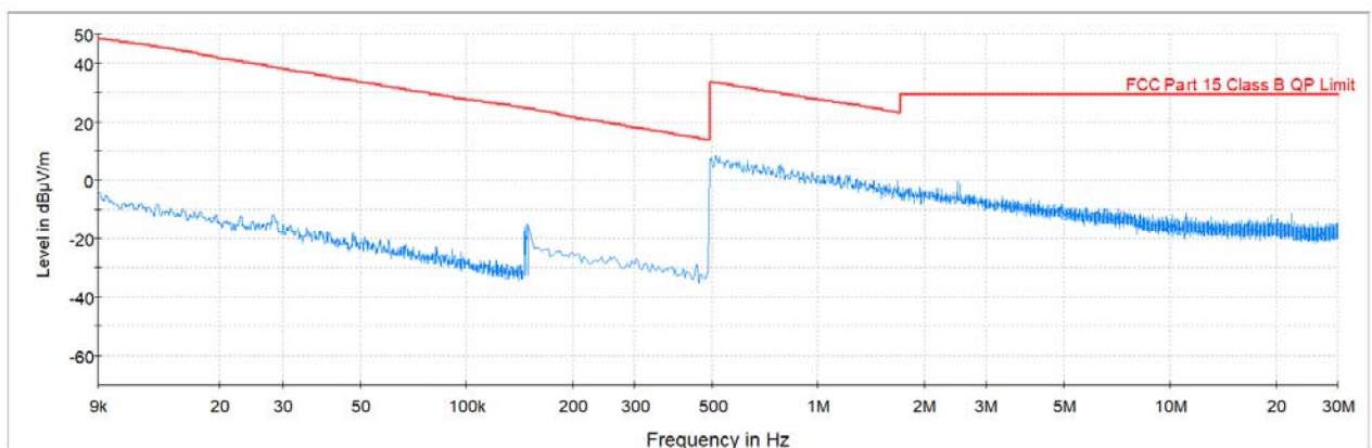
Plot 7-19. Radiated Spurious Plot from 9kHz – 30MHz (Pol. Z)
