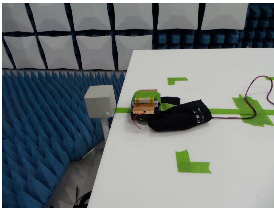
Figure 4. E-/H-Field Measurement (Position D)
