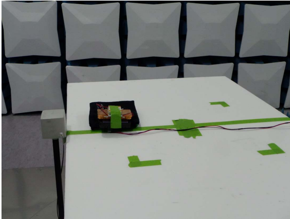
Figure 6. E-/H-Field Measurement (Position A)
