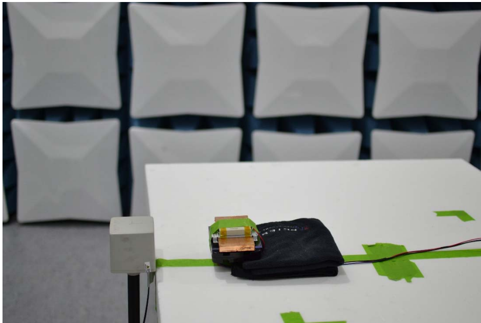
Figure 2. E-/H-Field Measurement (Position B)
