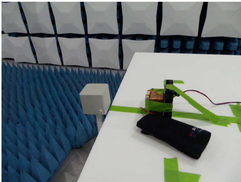
Figure 15. E-/H-Field Measurement (Position E)
