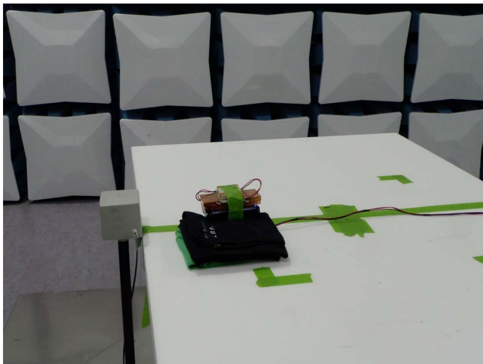
Figure 8. E-/H-Field Measurement (Position C)
