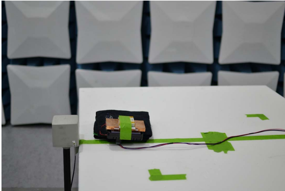
Figure 1. E-/H-Field Measurement (Position A)
