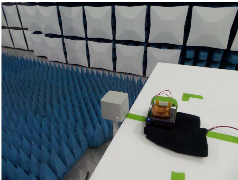
Figure 14. E-/H-Field Measurement (Position D)
