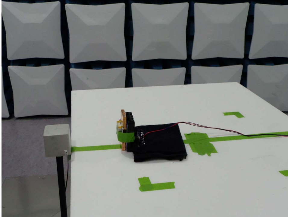
Figure 5. E-/H-Field Measurement (Position E)
