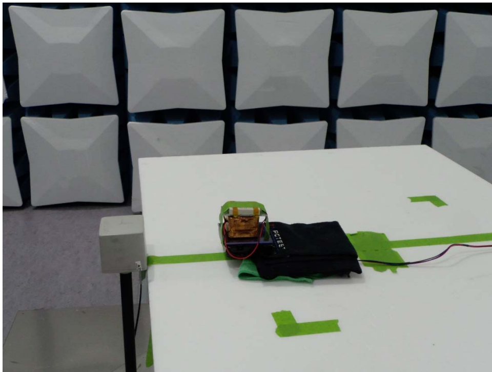
Figure 12. E-/H-Field Measurement (Position B)
