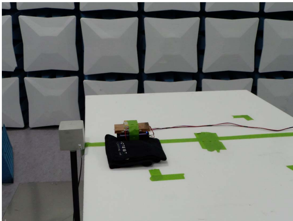
Figure 3. E-/H-Field Measurement (Position C)
