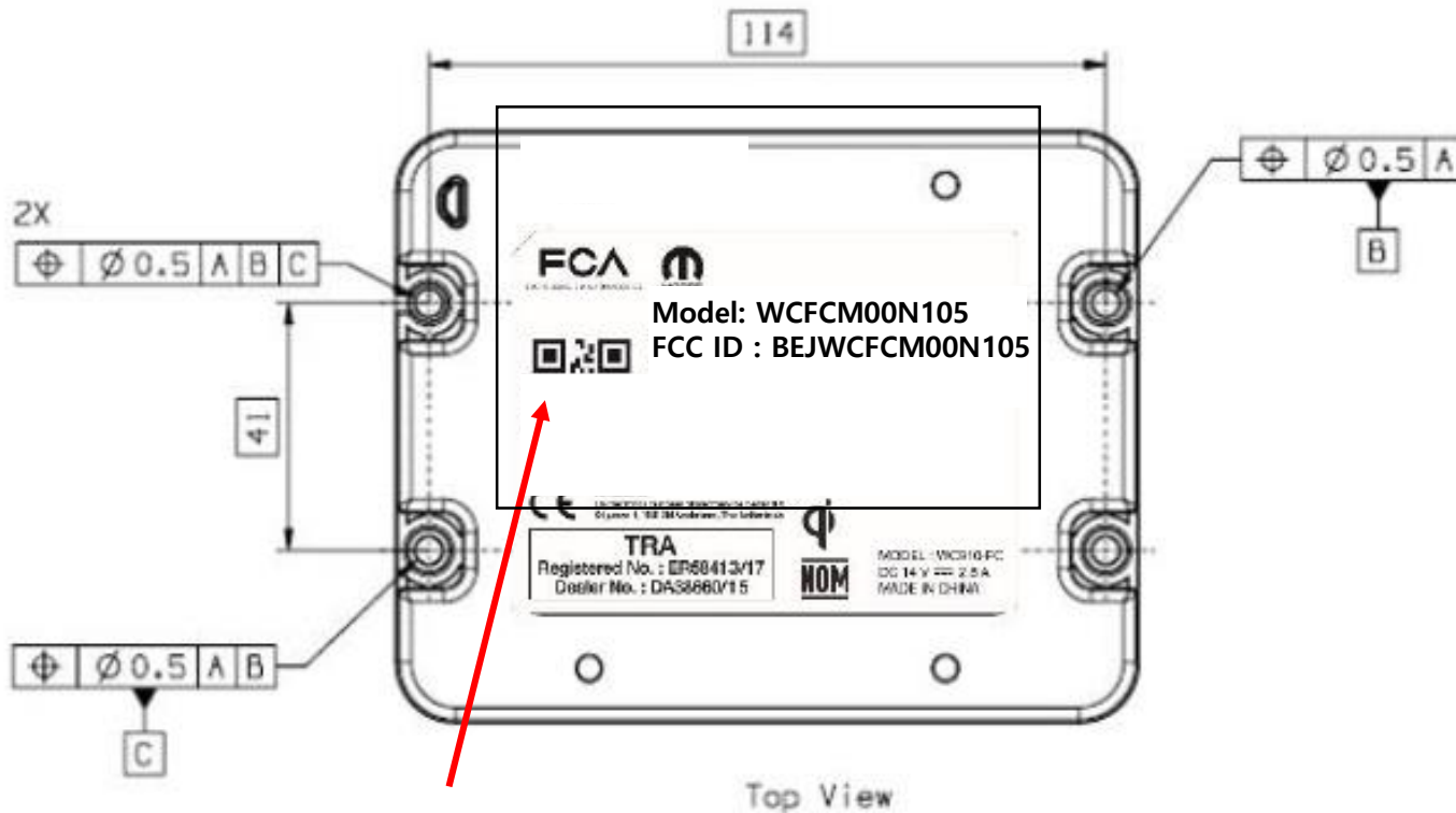
FCC ID Location (Top case)
