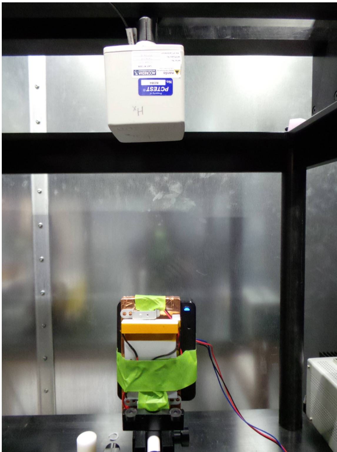
E/H Field Measurement on EUT Side “C”
