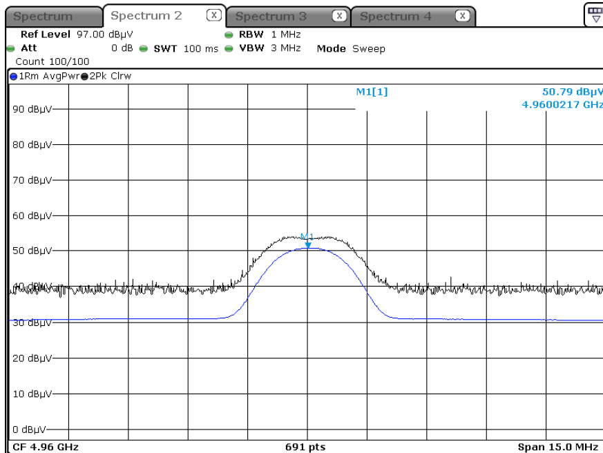
Radiated Spurious Emissions plot – Average Result (Ch.39 2nd Harmonic, X-H)
