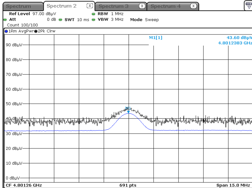
RECEIVER SPURIOUS EMISSIONS plot – Average Result (Ch.0 2nd Harmonic, X-H)
