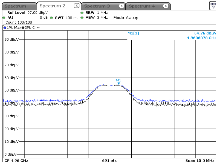
Radiated Spurious Emissions plot – Peak Result (Ch.39 2nd Harmonic, X-H)
