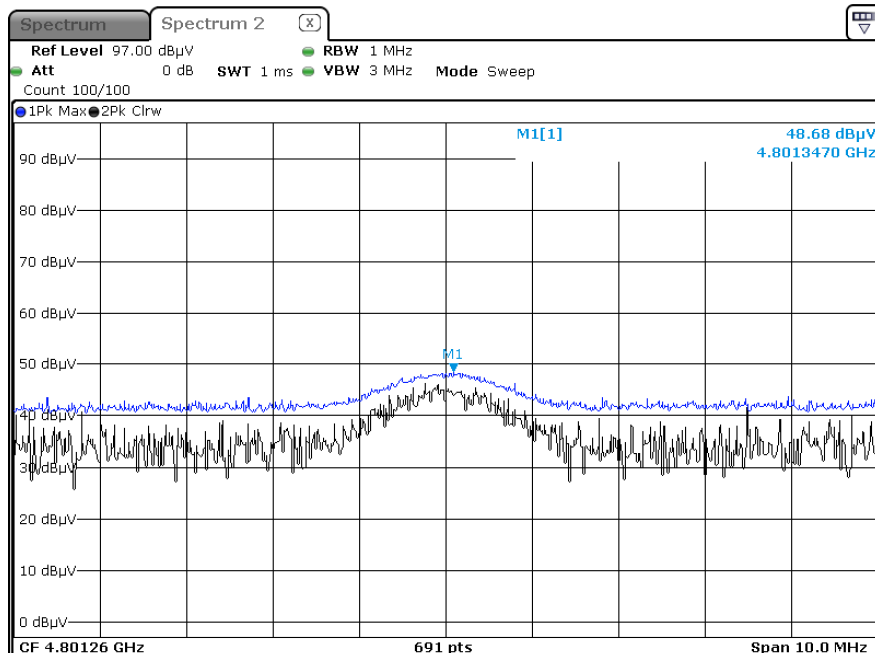
RECEIVER SPURIOUS EMISSIONS plot – Peak Result (Ch.0 2nd Harmonic, X-H)
