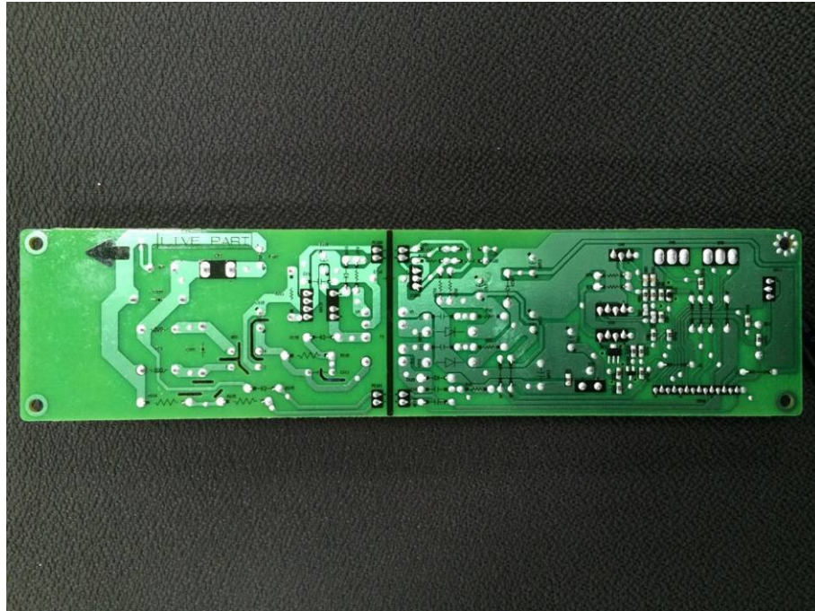
<PCB –Bottom of Power board>
