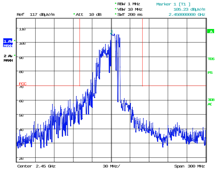
< Fig 10. Frequency Measurements (Minimum Frequency Observed: 2.445 GHz) >
