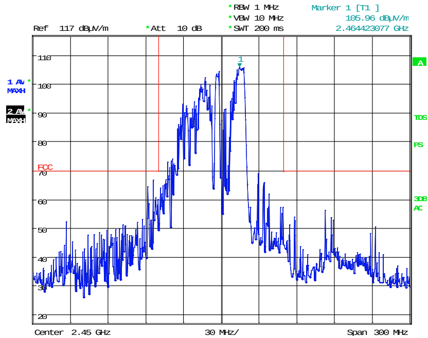
< Fig 9. Frequency Measurements (Maximum Frequency Observed: 2.464 GHz) >
