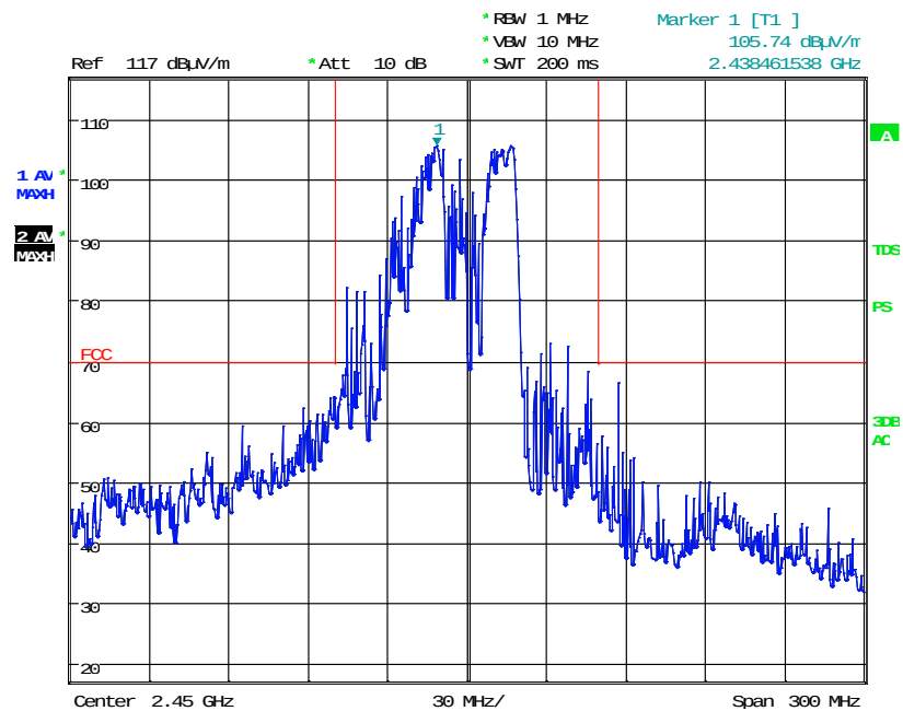
< Fig 8. Frequency Measurements (Minimum Frequency Observed: 2.438 GHz) >
