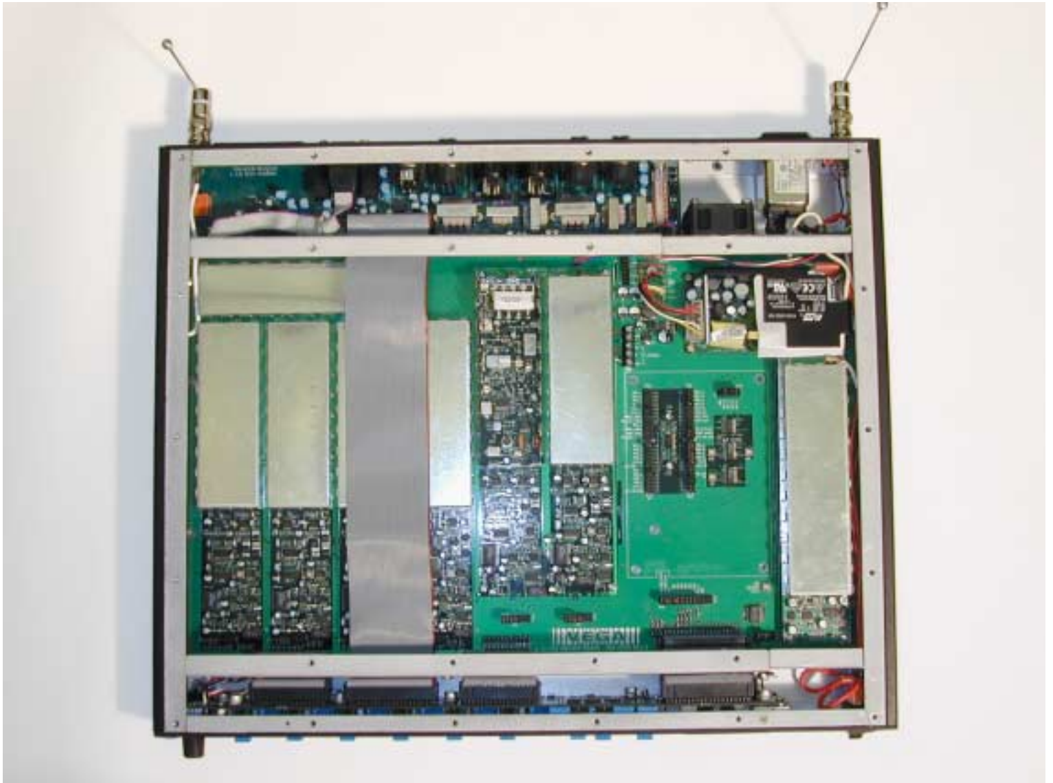
CHASSIS TOP
