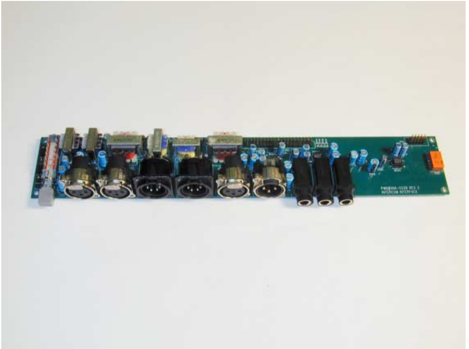
I/O, XLR ISOMETRIC
