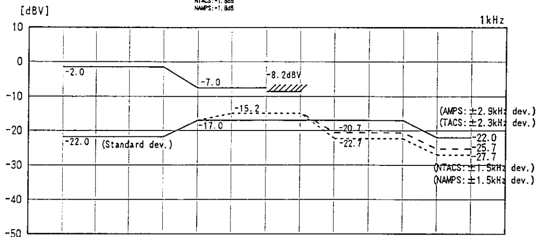
Transmit Voice Signal Level Diagram
