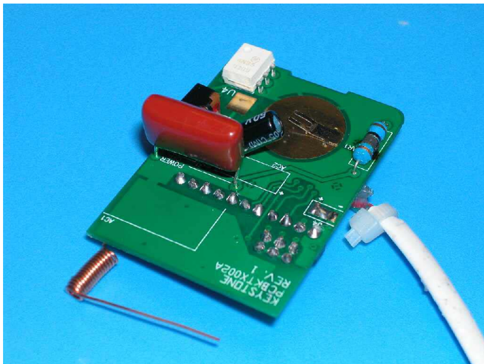
Internal Photo - 16
