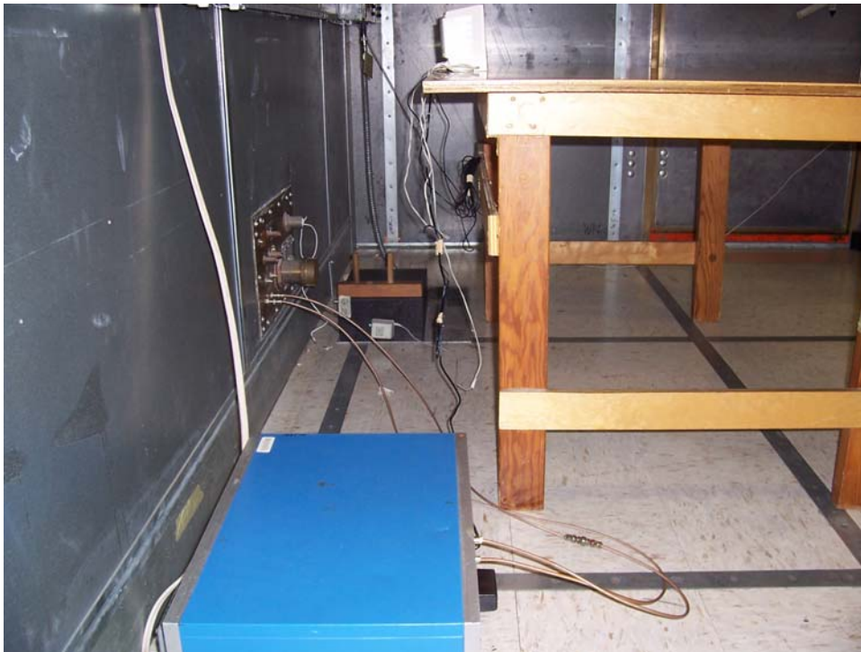
Conducted Emissions Test Setup, View 2
