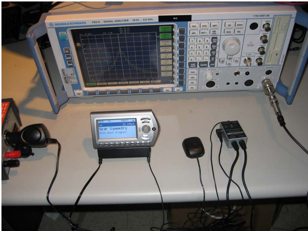
Photo 5 : Occupied Bandwidth
