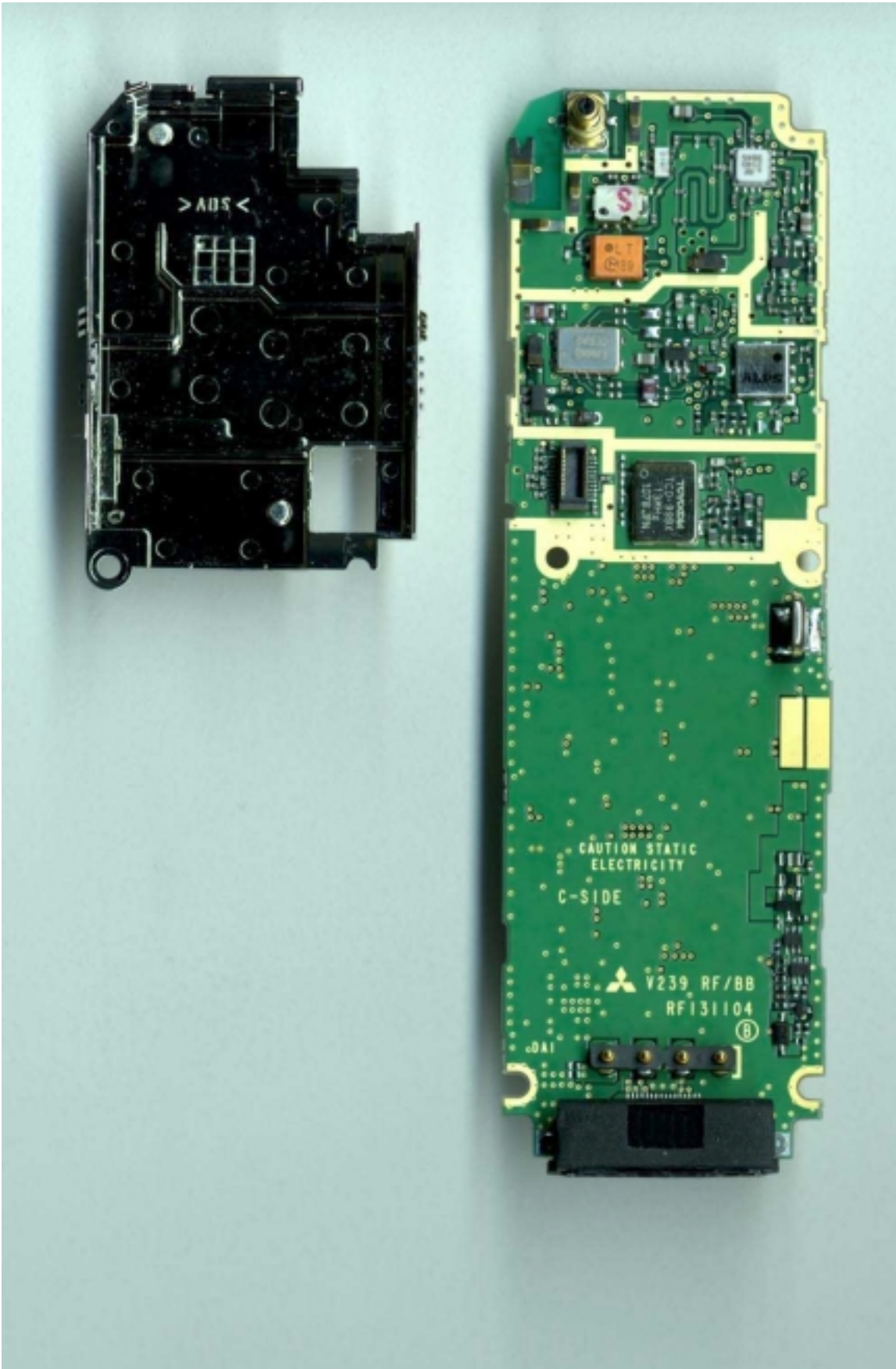
Photograph 8.11 Back PWB with Shield Removed
