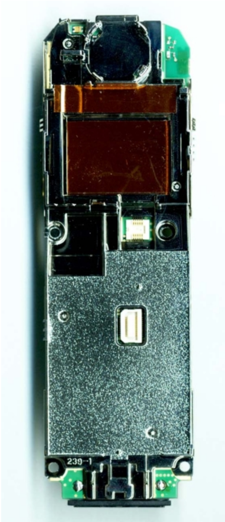
Photograph 8.9 Front PWB with Shield
