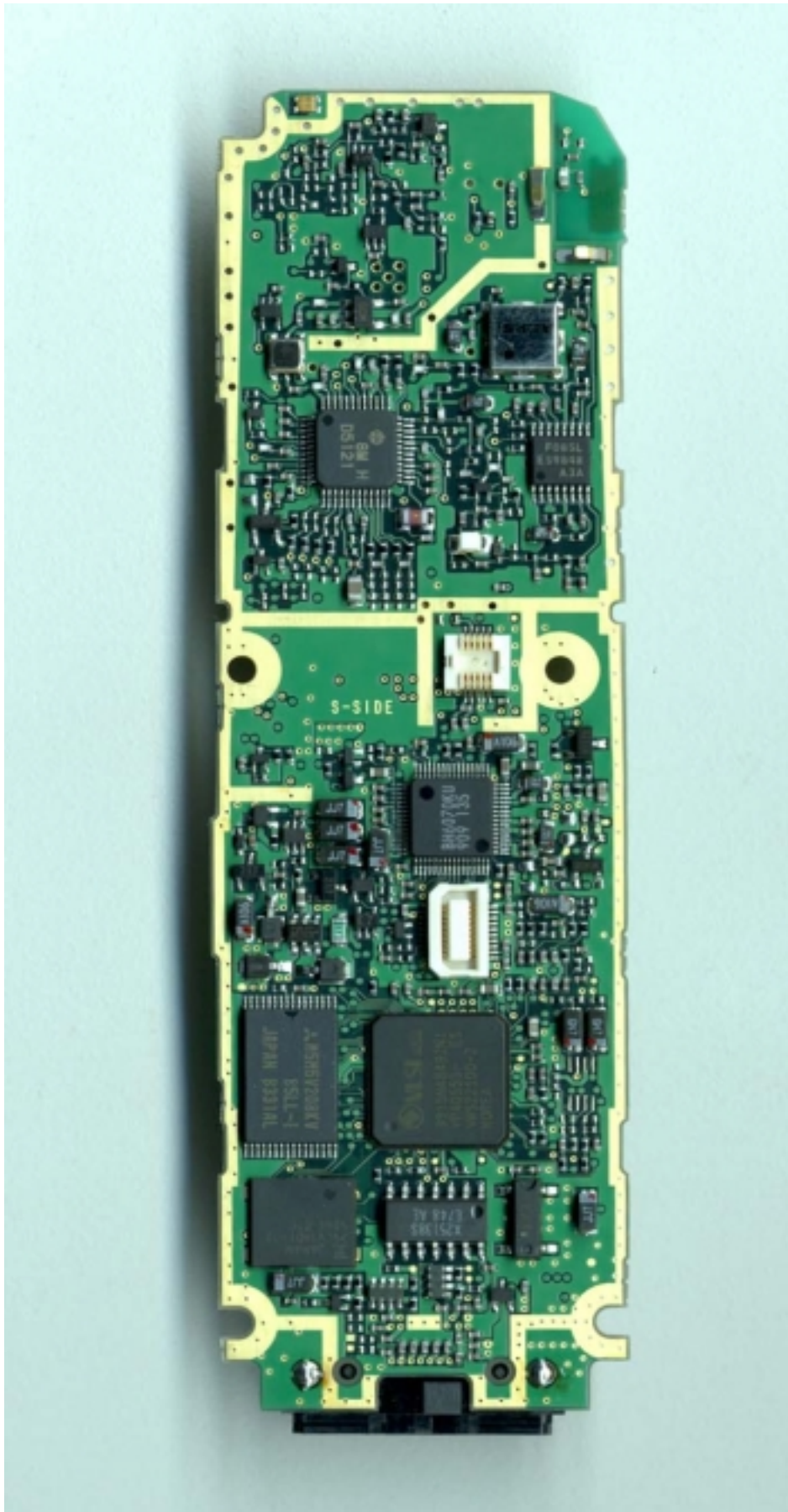
Photograph 8.12 Front PWB without Shield
