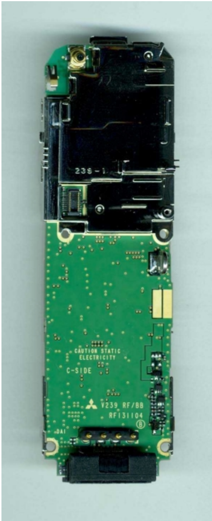
Photograph 8.10 Back PWB with Shields
