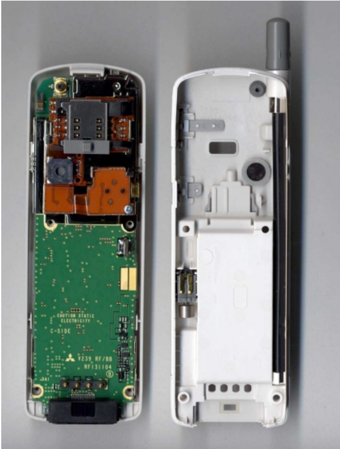
Photograph 8.7 MT-239XG01A (Back Cover Removed)
