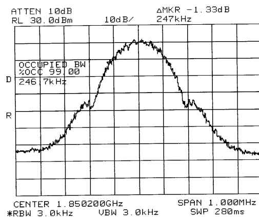
Figure 5.4.1 Block A Lower Edge 99% Power Occupied Bandwidth (Ch 512)
