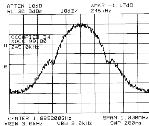
Figure 5.4.7 Block E Lower Edge 99% Power Occupied Bandwidth (Ch 687)
