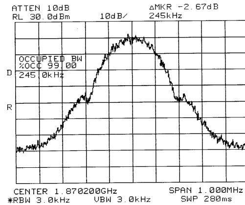
Figure 5.4.5 Block B Lower Edge 99% Power Occupied Bandwidth (Ch 612)
