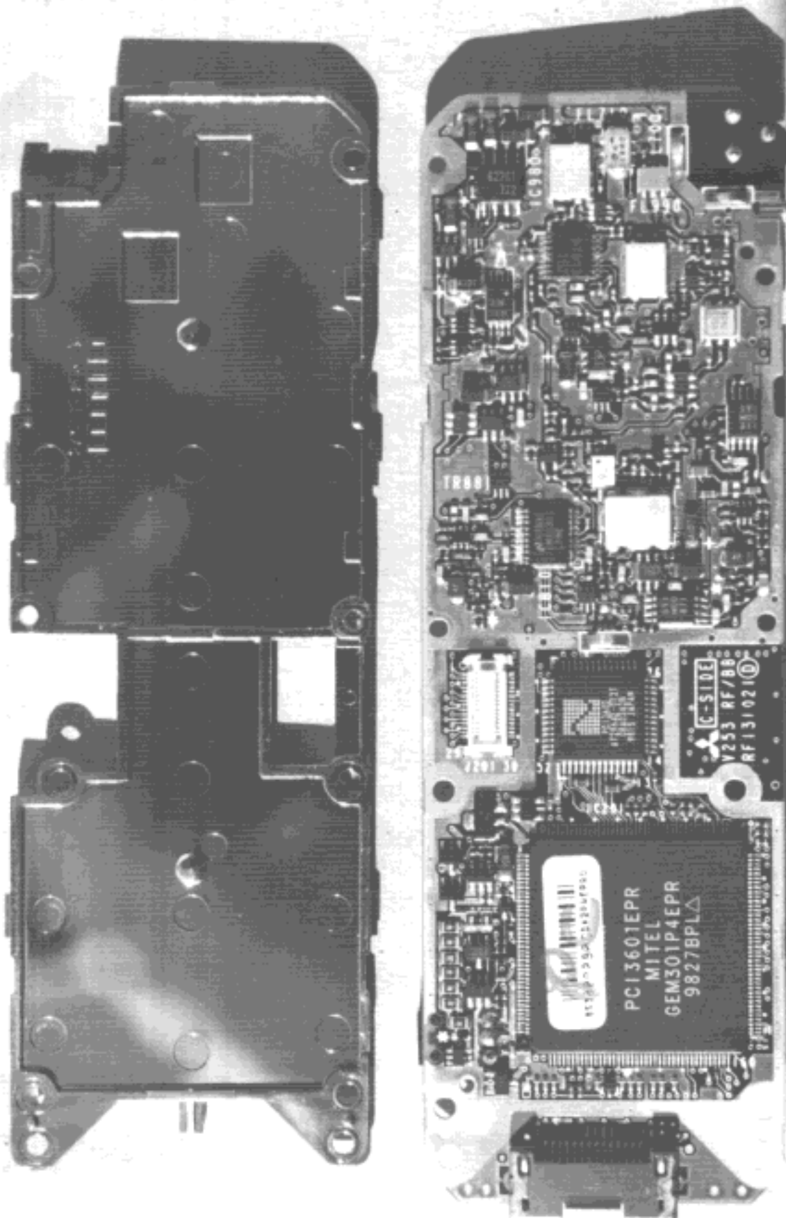
Photograph 8 RFBB board, C-side, shield detached
