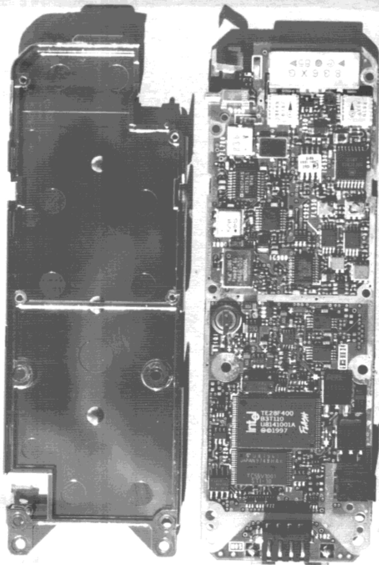
Photograph 9 RFBB board, S-side, shield detached
