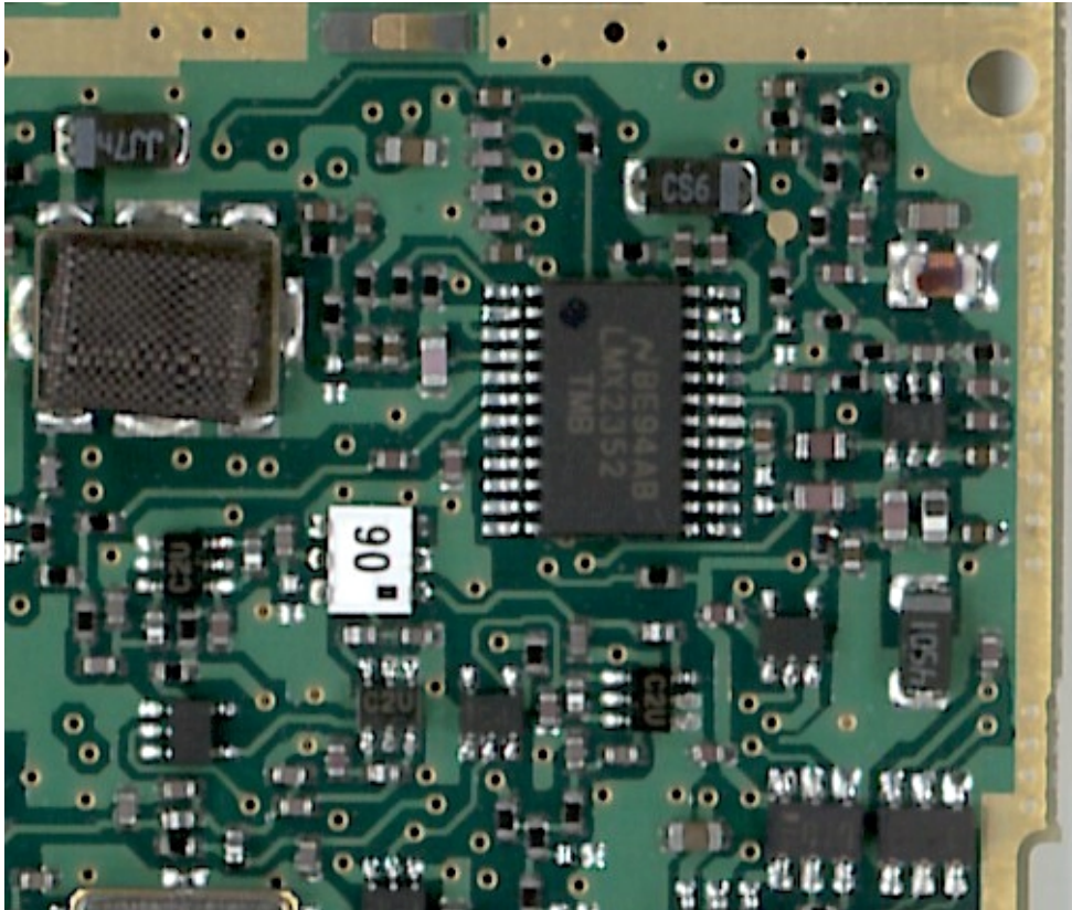
Photograph 1. LMX2352 Fractional N PLL Synthesizer
