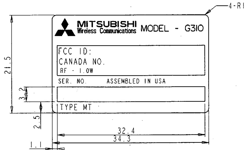
Figure 7.1.1 Identification Plate Drawing
