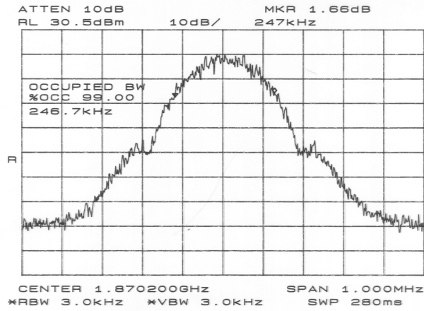
Figure 5.4.5 Block B Lower Edge 99% Power Occupied Bandwidth (Ch 612)
