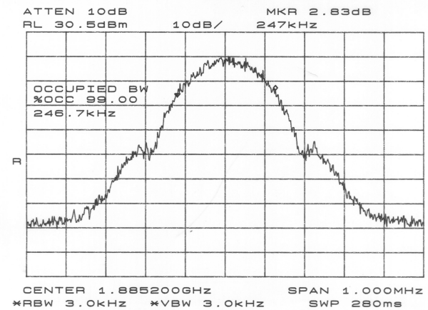
Figure 5.4.7 Block E Lower Edge 99% Power Occupied Bandwidth (Ch 687)
