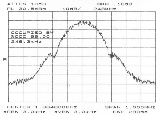
Figure 5.4.6 Block B Upper Edge 99% Power Occupied Bandwidth (Ch 685)
