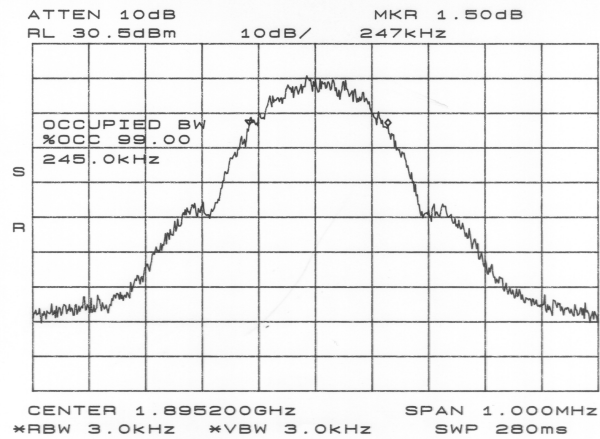
Figure 5.4.11 Block C Lower Edge 99% Power Occupied Bandwidth (Ch 737)
