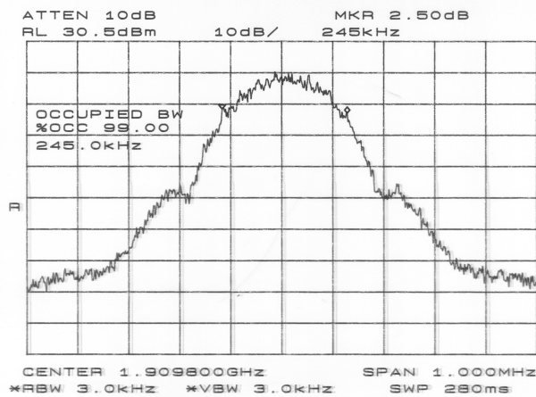
Figure 5.4.12 Block C Upper Edge 99% Power Occupied Bandwidth (Ch 810)
