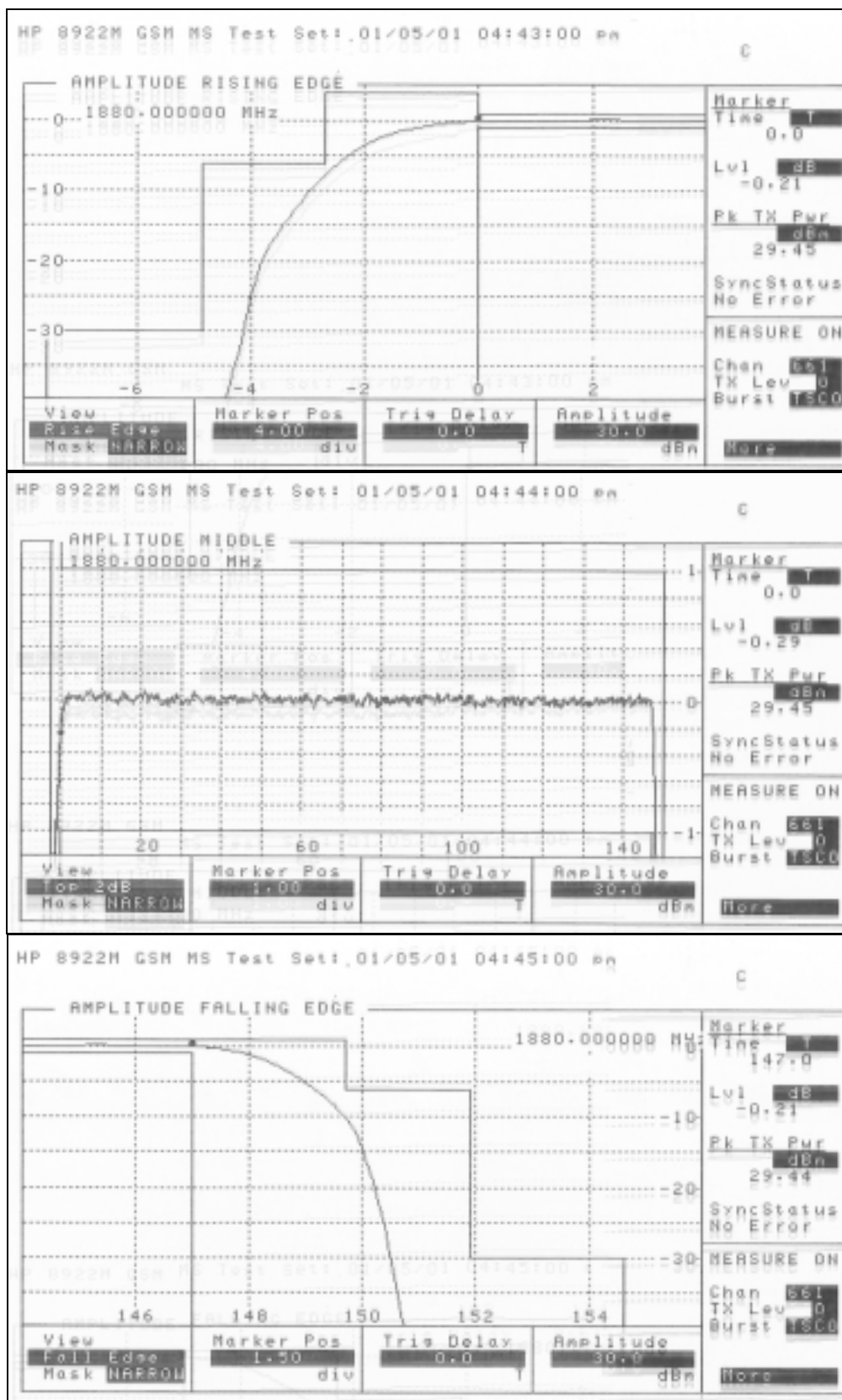
Figure 6.2.4 Carrier 1880.0 MHz (Ch 661) Power Level 0
