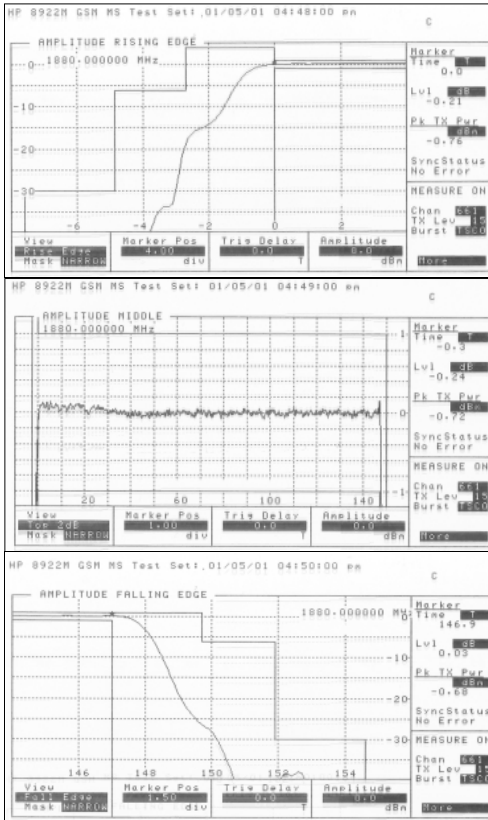
Figure 6.2.6 Carrier 1880.0 MHz (Ch 661) Power Level 15
