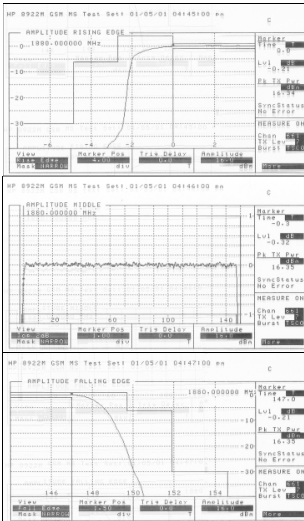
Figure 6.2.5 Carrier 1880.0 MHz (Ch 661) Power Level 7
