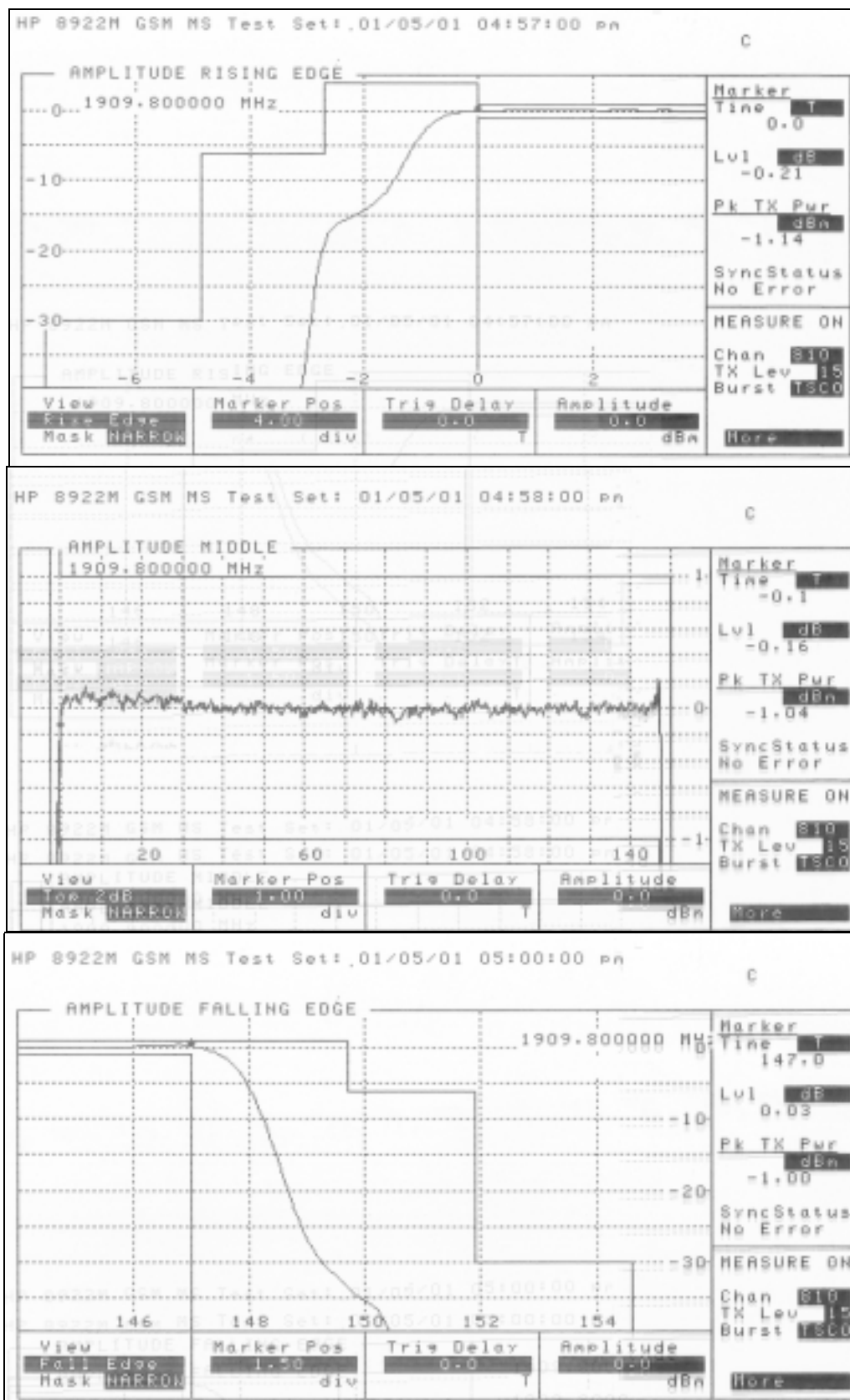
Figure 6.2.9 Carrier 1909.8 MHz (Ch 810) Power Level 15
