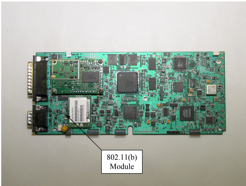
Figure 5C-1 CMU Board, top, with 802.11(b) module installed
