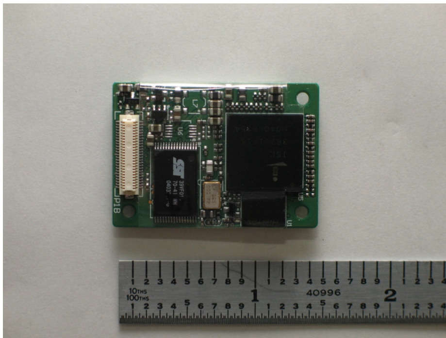
Figure 5C-1 DPAC 802.11(b) Board, top
