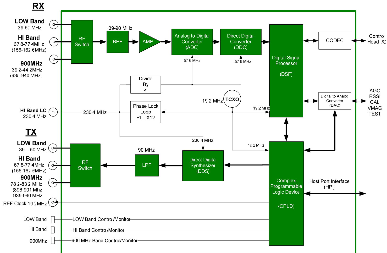
MCC-6100 DIGITAL SIGNAL PROCESSOR (DSP) BLOCK DIAGRAM FIGURE 2.2-3
