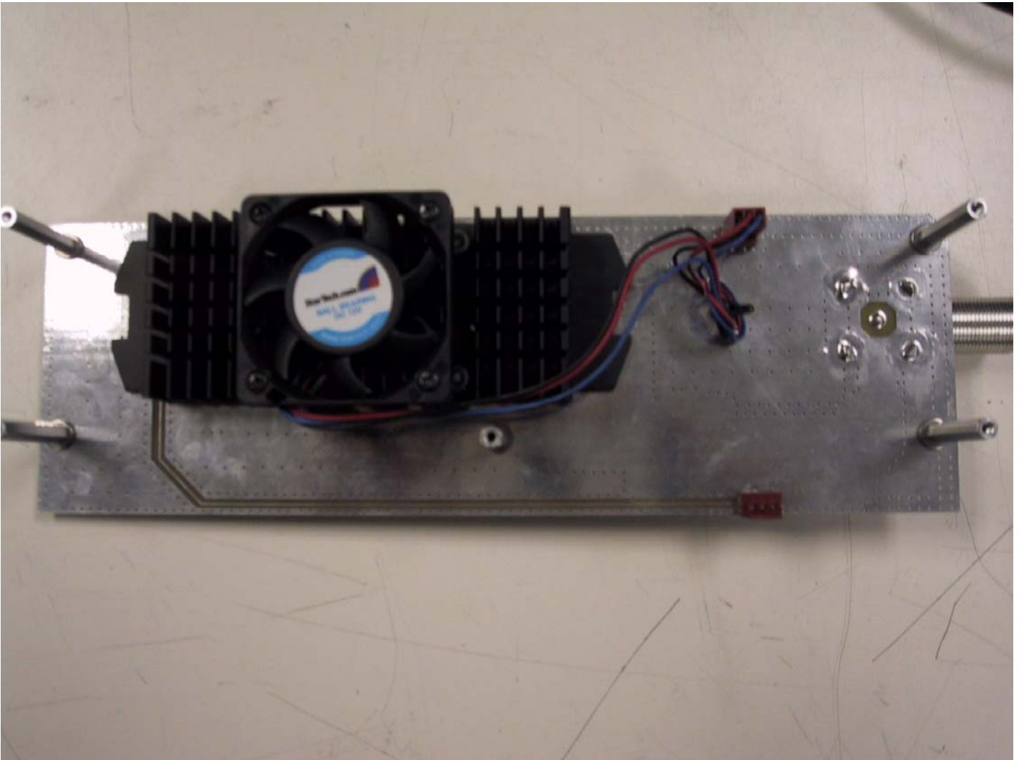
Power Amp PCB – Bottom
