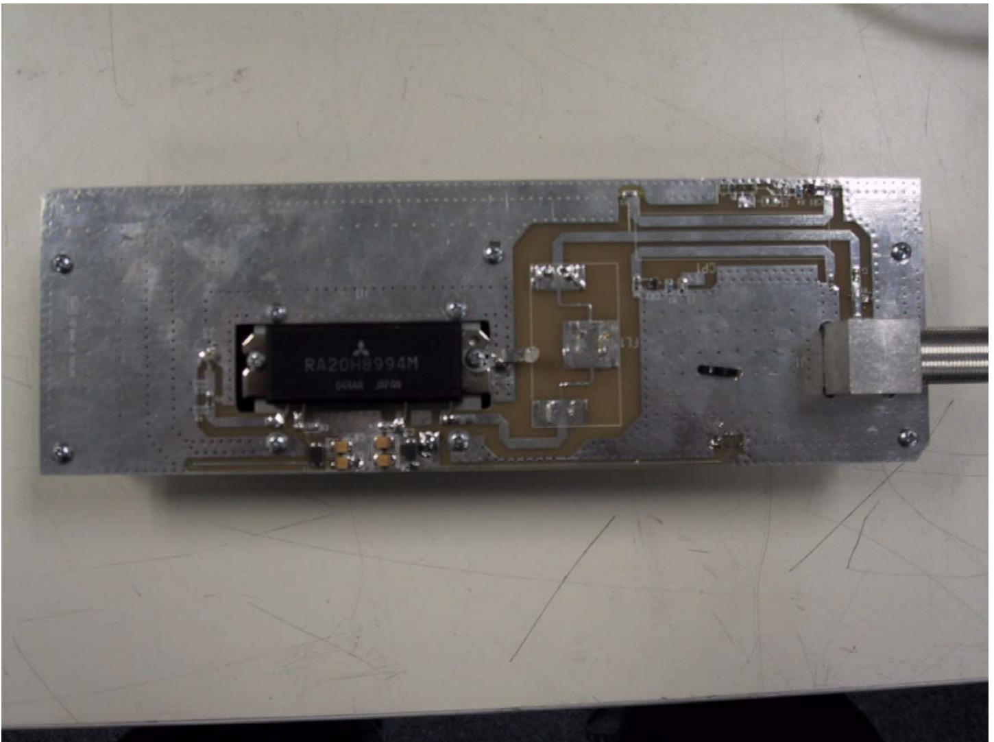
Power Amp PCB – Top
