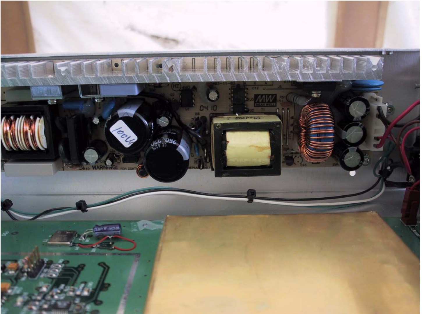
Power supply PCB - Installed
