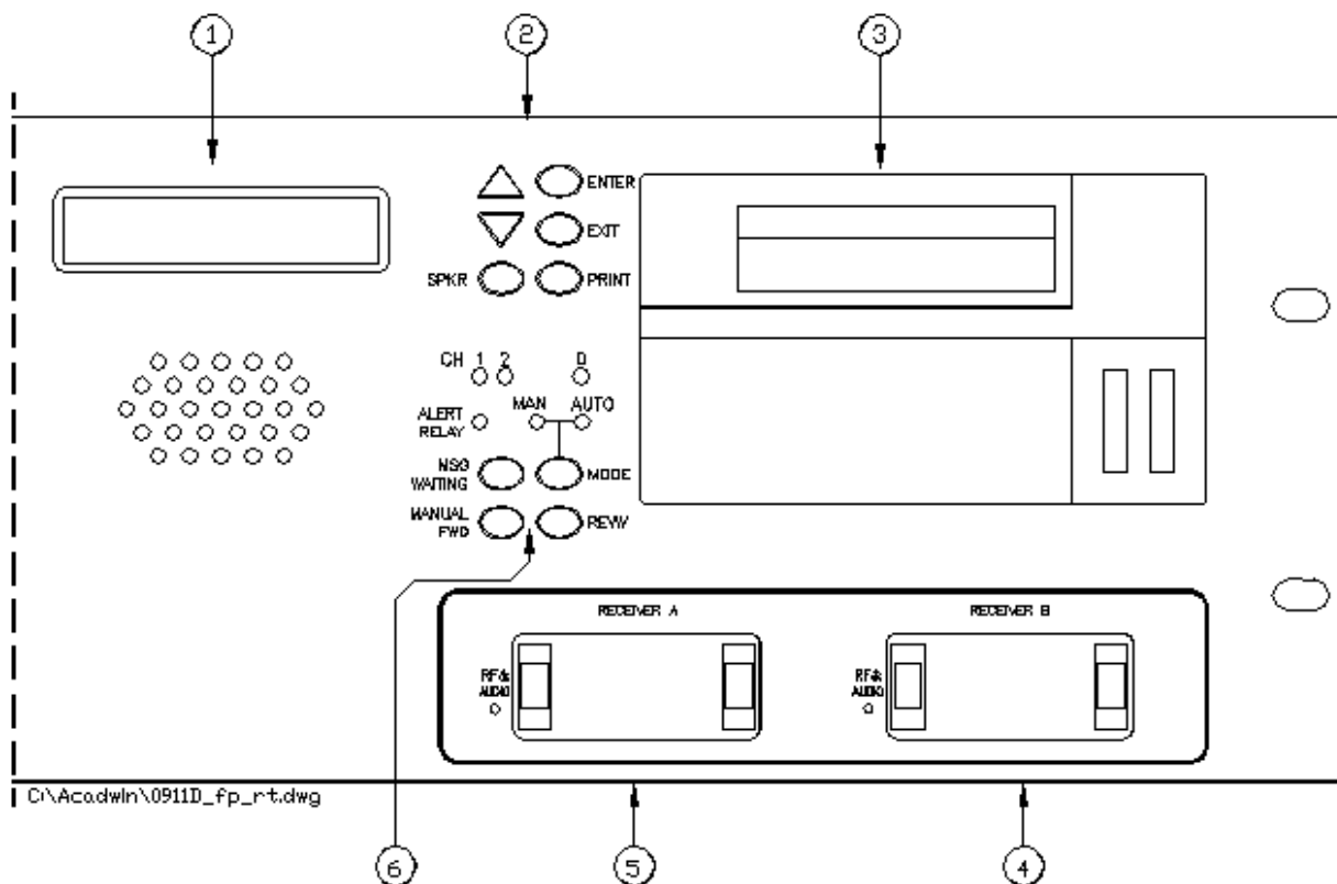
Figure 2.3-2. Decoder Controls and Indicators
