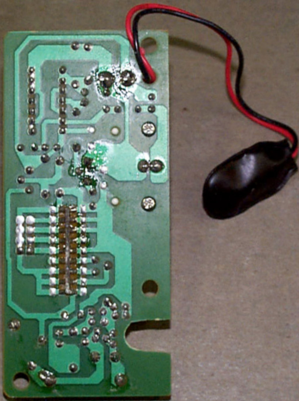
PCB Back
