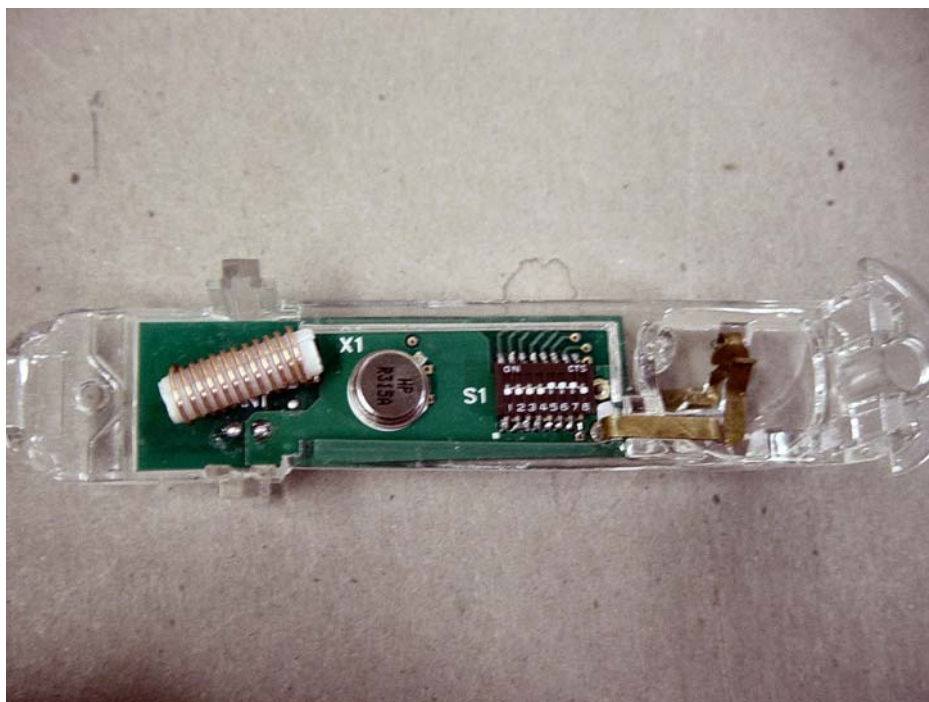
EUT with Helix Antenna view
