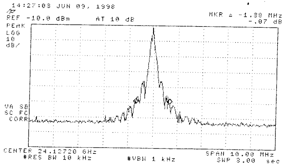
Figure 6.1. Fundamental emission spectrum.
