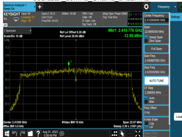
802.11ax 20MHz Chain1 2412MHz RU106_53
