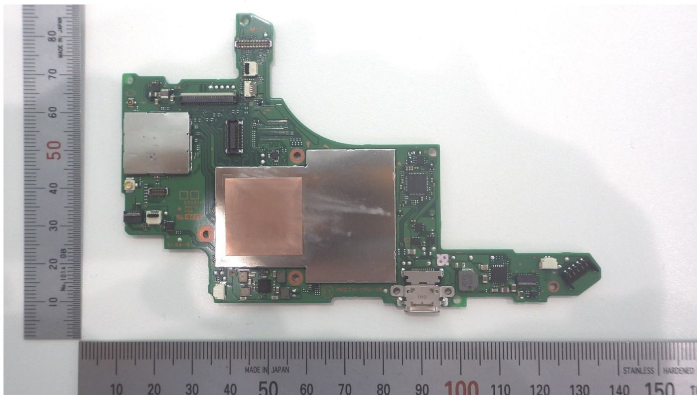
Wireless module PCB (Front, Shielded):
