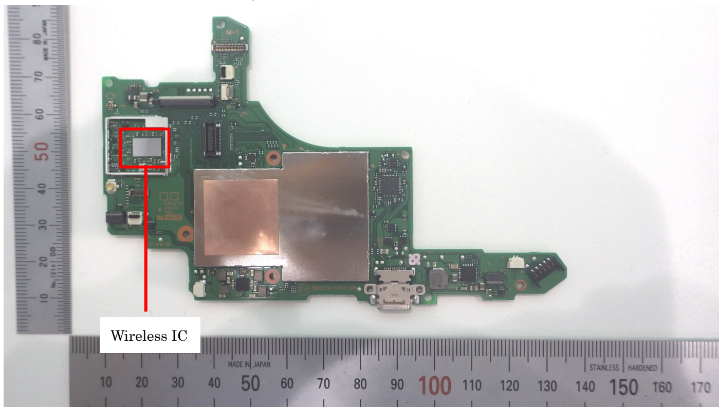
Wireless module PCB (Front, Shield removed):
