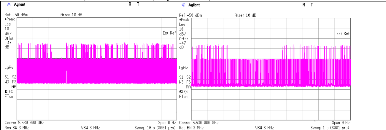
Plots of WLAN Traffic (11ac VHT80, MIMO, duty about 18 %)
