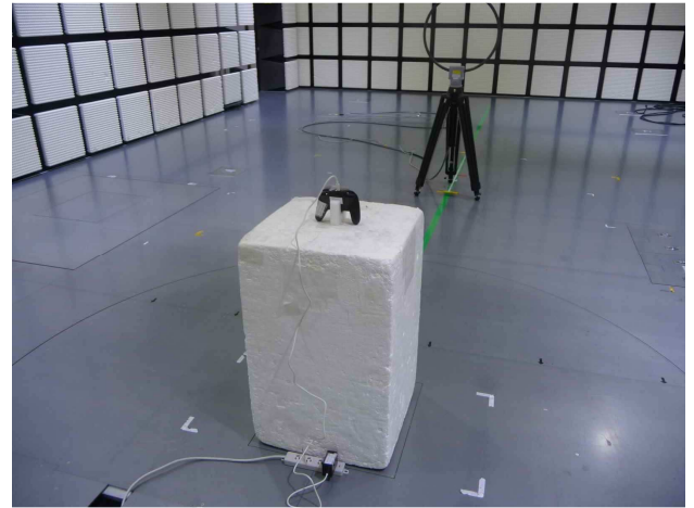
Rear (below 30 MHz, antenna vertical)
