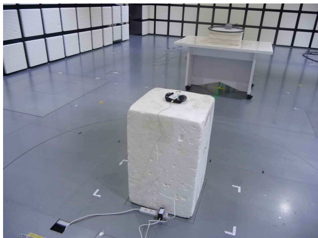
Rear (below 30 MHz, antenna horizontal)
