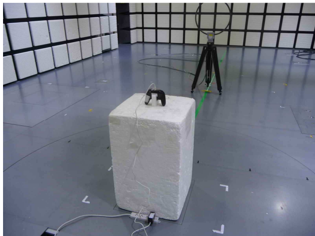
Rear (below 30 MHz, antenna vertical)
