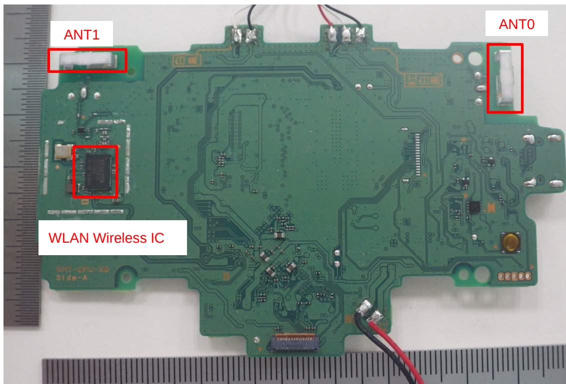
Wireless module PCB (Front, Shield removed):
