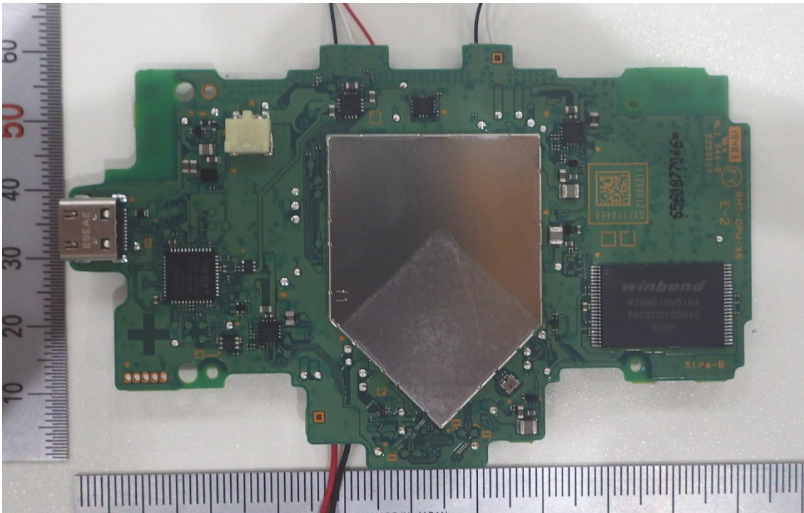
Wireless module PCB (Back):
