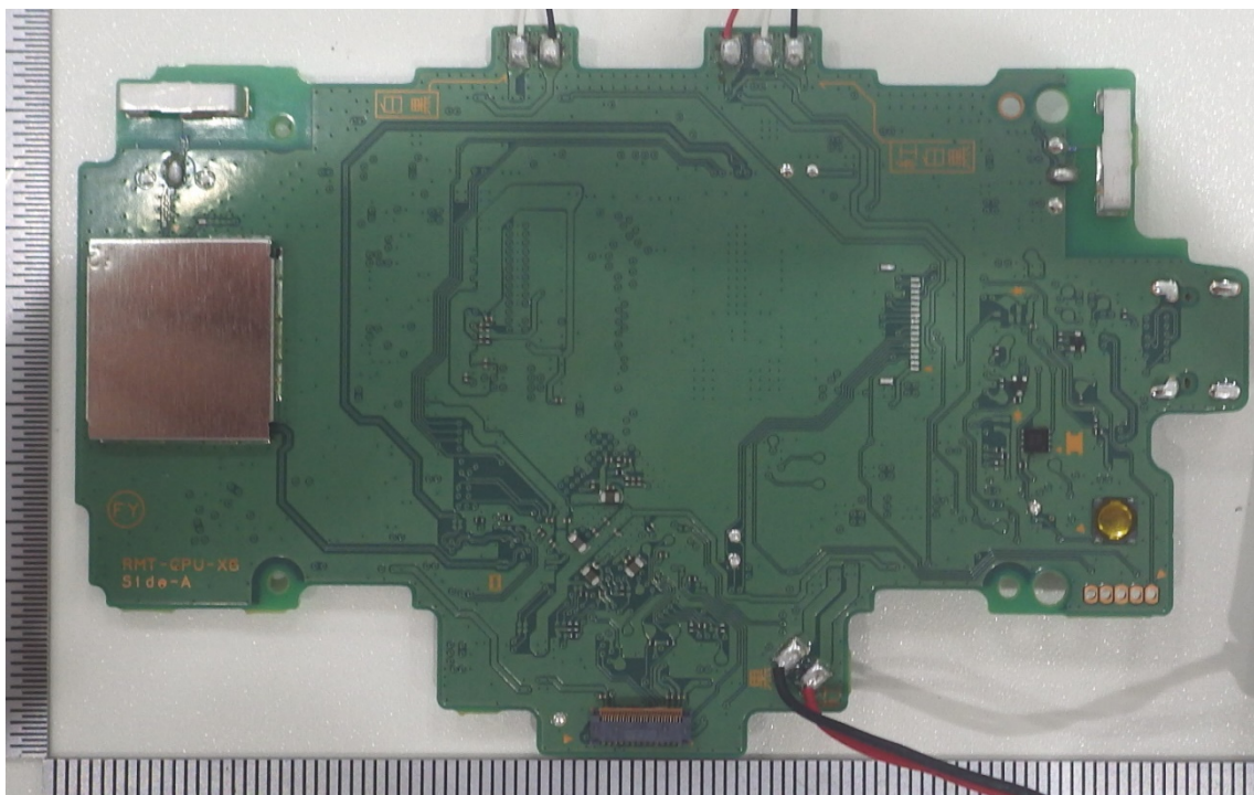
Wireless module PCB (Front, Shielded):
