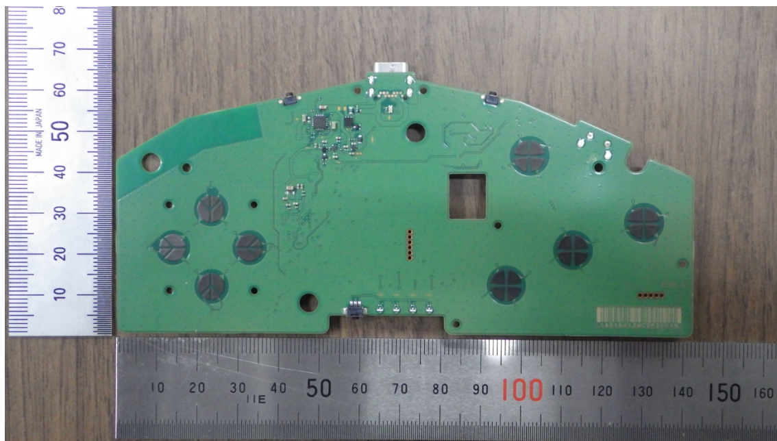
Wireless module PCB (Front):
