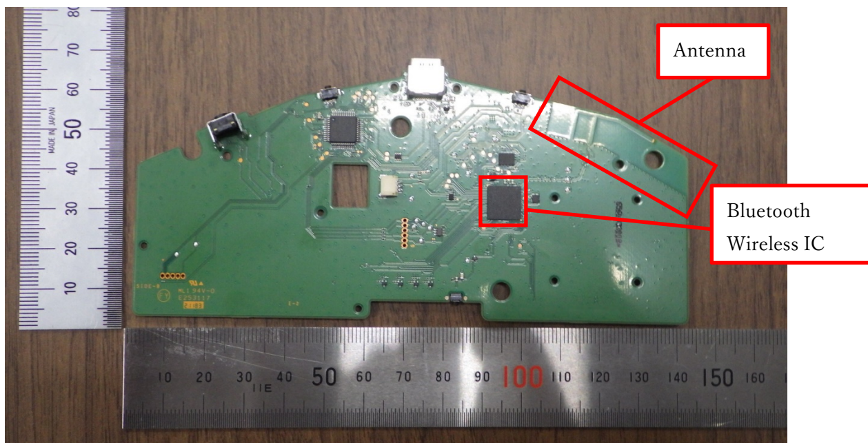
Wireless module PCB (Back):
