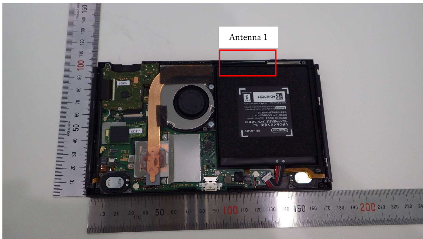
Antenna location (Rear)
