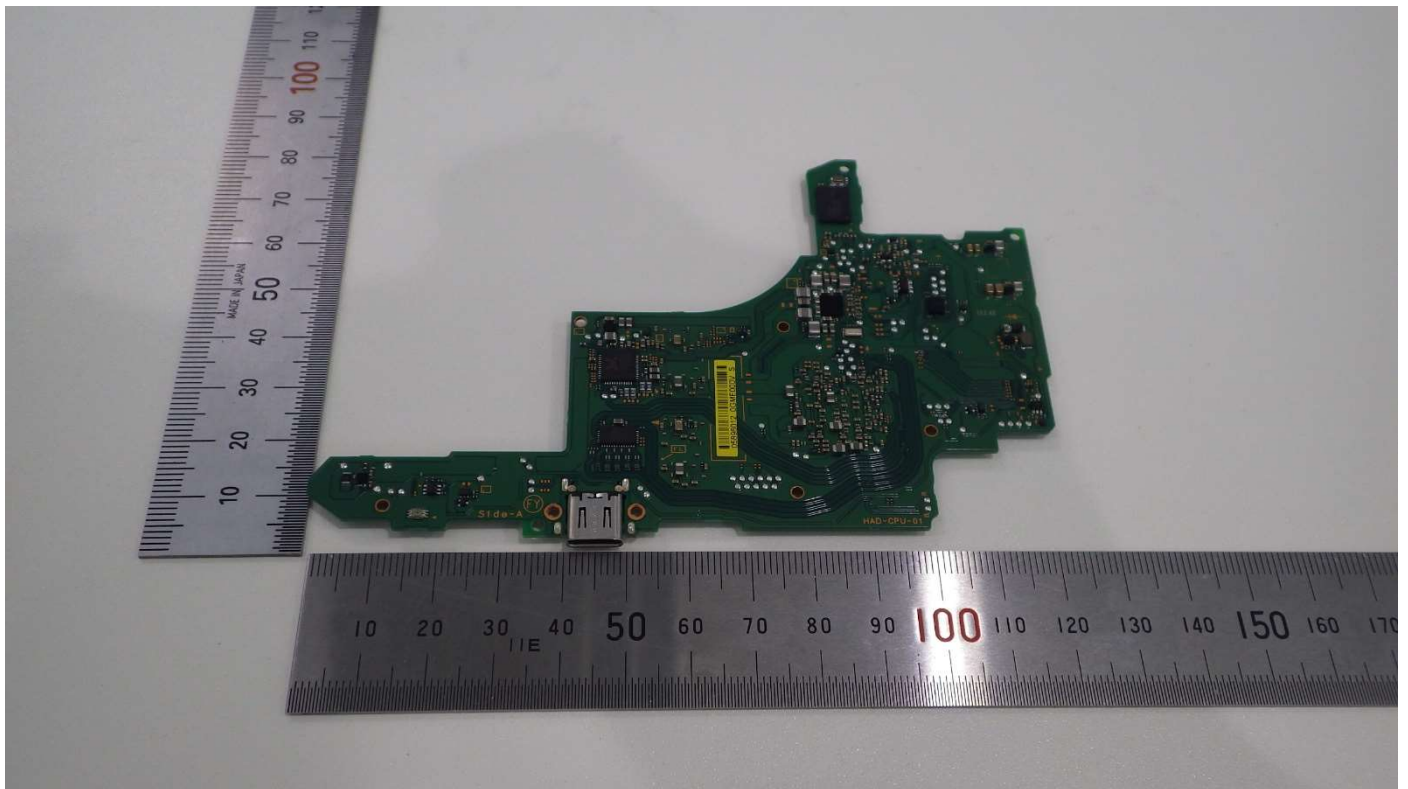
Wireless module PCB (Back)
