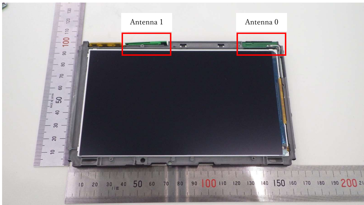
Antenna location (Front)
