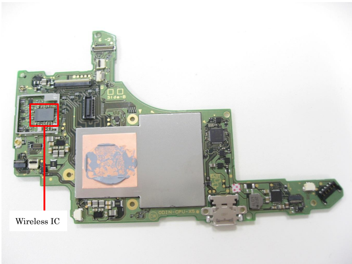
Wireless module PCB (Front, Shield removed):
