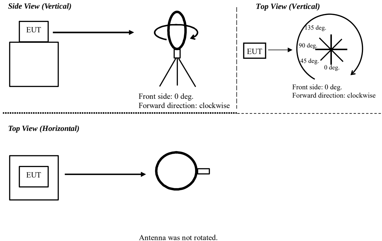
Figure 2: Direction of the Loop Antenna
